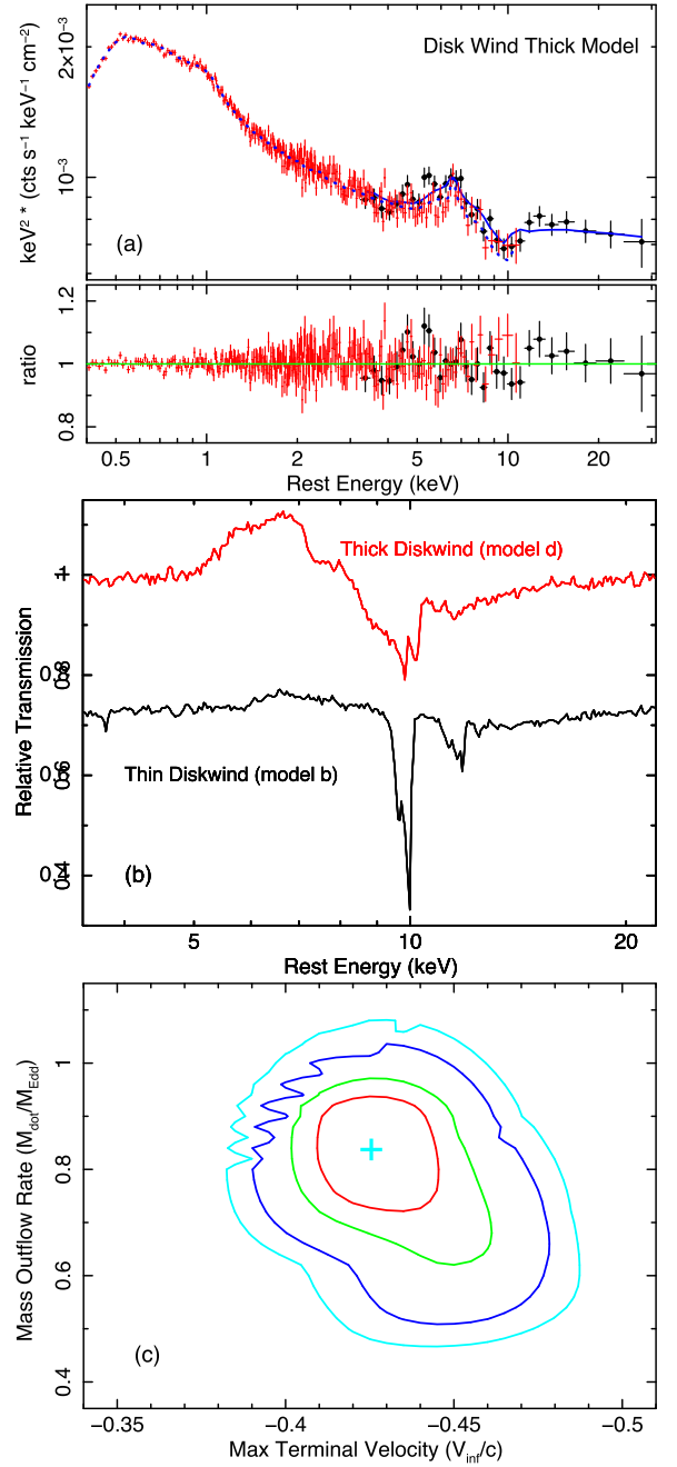
Figure 7. Results of the disk-wind modeling. Panel (a) shows the best-fit DW thick model fitted to the mean 2023 spectrum. Here, the model (folded through the instrumental responses) is shown as a solid blue line fitted to the NuSTAR data from 3 to 30 keV and as a dotted blue line to the XMM-Newton spectrum from 0.3 to 10 keV. Note the lack of strong soft-X-ray absorption. Panel (b) shows the theoretical Fe K profiles predicted from the wind for the DW thick case (red; Table 2, model (d)) vs. the DW thin case (black; Table 2, model (b)). A y-axis offset has been applied for clarity. The DW thick model produces a broader absorption-line profile due to its larger velocity shear, as well as stronger Fe K emission. Panel (c) shows the confidence contours of the mass outflow rate in Eddington units vs. the maximum terminal velocity attained by the wind for model (d). The contours represent the 68%, 90%, 99%, and 99.9% confidence levels for two interesting parameters. The mass outflow rate in PG1448+273 appears to be at nearly the Eddington rate, with a maximum terminal velocity of v_{\max,\infty}/c = -0.43 \pm 0.03 . Note the sawtooth behavior of the outer contours is due to the finite grid resolution.
