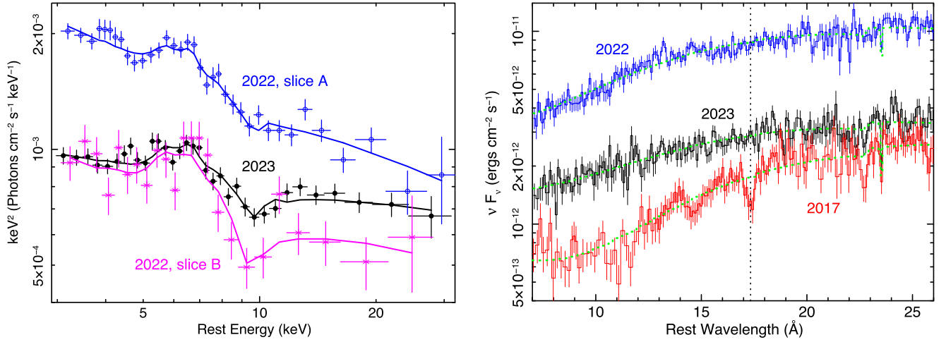
Figure 9. Comparison of the PG1448+273 spectra over different epochs from 2017 to 2023. The left panel shows the the mean 2023 vs. the 2022 A (slice A) and 2022 B (slice B) NuSTAR spectra, fitted with the thick disk-wind model in each case. The spectral differences between each epoch can be accounted for via changes in ionization through the variations in X-ray luminosity, as well as in photon index. Note there was no NuSTAR observation in 2017. The right panel shows the comparison of the 2017, 2022, and 2023 RGS spectra. Significant soft-X-ray wind absorption was only detected in the low-flux 2017 spectrum, in the form of a blueshifted O VIII Ly \alpha line, as marked by the dotted vertical line.
