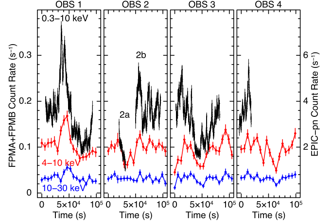
Figure 2. Background-subtracted lightcurves from the 2023 XMM-Newton and NuSTAR observations of PG1448+273. The x-axis shows the time elapsed for each observation, compared to the start time of each NuSTAR exposure, while the y-axis shows the count rates for NuSTAR (FPMA+FPMB) and EPIC-pn (right-hand axis). The 0.3–10 keV EPIC-pn lightcurve is shown in black in 200 s bins, while NuSTAR is shown in red and blue, over the 4–10 keV and 10–30 keV bands, respectively, and are binned into 5814 s orbital bins. Note the gap in XMM-Newton OBS 2, split into two sequences (2a and 2b as marked), was due to the solar flare which interrupted the observation. Overall, the average source flux was similar between each of the observations, while a notable flare was observed in OBS 1 and OBS 2a appears to coincide with a short dip in the lightcurve. The variability amplitude in the hardest 10–30 keV band is modest in comparison.
