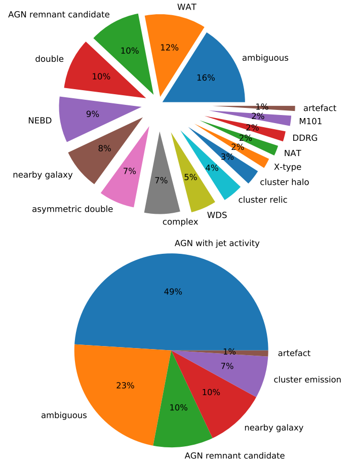
Fig. 11: Piechart showing the wide variety of morphologies and radio source types present in the 100 most outlying sources in the final 10 \times 10 cyclic SOM. Top panel: Descriptive labels have been established by a manual visual inspection of each source in radio (LoTSS), mid-infrared (WISE) and optical (SDSS9 colour). We labelled sources that fitted in more than one category as ‘ambiguous’. ‘X-type’ sources are ‘X-shaped’ extended doubles (Rees 1978), ‘WATs’ and ‘NATs’ are Wide Angle Tailed and Narrow Angle Tailed sources, ‘WDS’ are Wide Double Sources, ‘NEBD’ are Narrow Edge Brightened Doubles (Miley 1980), ‘DDRG’ are Double-Double Radio Galaxies (Schoenmakers et al. 1999). An ‘AGN remnant candidate’ is an extended double with such relaxed morphology that the AGN jets might not be active any more. As M101 is an exceptionally large apparent object, the source detection software did not group the separate detections of this nearby spiral, as a result it features multiple times in the catalogue. Bottom panel: We grouped subtypes together to get an overview of the dominant types of sources in the outliers: ‘M101’ was grouped with ‘nearby galaxy’; ‘complex’ with ‘ambiguous’; ‘cluster relic’ and ‘cluster halo’ were grouped into ‘cluster emission’ and ‘DDRG’, ‘NEBD’, ‘NAT’, ‘WAT’, ‘WDS’, ‘double’, ‘asymmetric double’ and ‘X-type’ were grouped into ‘AGN with jet activity’. A figure containing each of these one hundred most outlying sources can be found in Appendix B.
