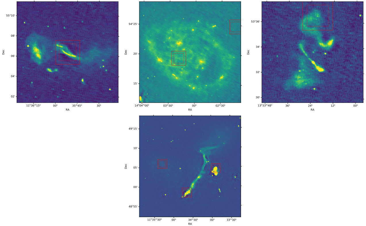
Fig. 12: Continued: The outliers list contains a wide range of objects. Going row by row from left to right: an AGN remnant candidate (Shulevski et al in prep.), M101, diffuse emission combined with AGN emission, diffuse emission next to a giant head-tail AGN next to a WAT (Wilber et al. 2019). As the source extraction and association software PyBDSF did not associate radio emission of objects with a large (greater than a few hundred arcsec) apparent size, these appear as multiple separate entries in the source catalogue. The SOM can thus give different parts of the same astronomical object a high outlier score. We adopt a minimum separation distance between outlying objects of 400 arcsec.
