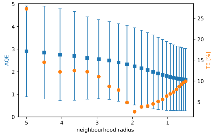
Fig. 3: Training process of the final 10 \times 10 cyclic SOM. Neighbourhood radius is the radius on the SOM lattice. With each epoch we decrease the neighbourhood radius which results in an increasingly accurate SOM (lower AQE) and higher coherency (lower TE). Eventually we increase the accuracy at the cost of the coherency (higher TE). As the AQE is the average of the Euclidean norm between each cutout and its best matching neuron, the errorbars indicate the standard deviation of these values for our data set.
