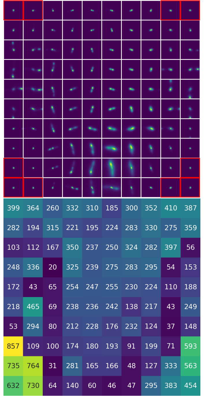
Fig. A.1: Top panel : First run 10×10 cyclic SOM. The first run reveals that our preprocessed dataset still contains a large fraction of unresolved sources. We remove these from the training dataset by removing all radio sources that map to one of the red highlighted representative images. Bottom panel : Heatmap of the first run SOM, indicating the number of sources mapped to each of the representative images.
