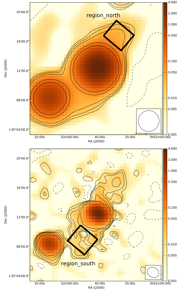
Fig. 3. Top panel: LOFAR image at 145 MHz convolved to 2.9-arcmin resolution. Contours represent -2, 2, 3, 5, 10, 20 \times \sigma ( 5 \text{ mJy beam}^{-1} ). Bottom panel: LOFAR image at 145 MHz and 80 \text{ arcsec} \times 98 \text{ arcsec} resolution. Contours represent -2, 2, 3, 5, 10, 20 \times \sigma ( 3 \text{ mJy beam}^{-1} ). The black regions represent the boxes used to extract the flux density in the northern lobe and southern lobe respectively. The colour scale is set in \text{Jy beam}^{-1} .
