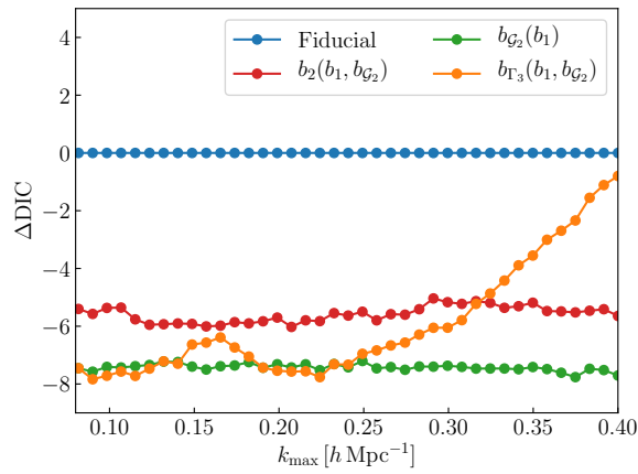
Figure 10. Difference in DIC, with respect to the fiducial case, of the alternative models that assume relations between bias parameters, as a function of k_{\max} , for an effective volume of 6 h^{-3} \text{Gpc}^3 .
