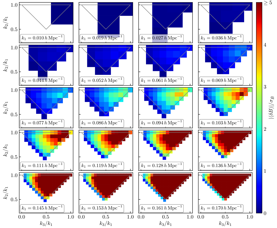
Figure 13. Mean residuals, normalized to the standard error on the mean, of all the measured bispectrum bins, assuming the posterior-averaged tree-level model of the reference analysis, k_{\max, \text{P}} = 0.30 h \text{ Mpc}^{-1} , k_{\max, \text{B}} = 0.09 h \text{ Mpc}^{-1} . In each panel, we fix the value of k_1 and show all triangle bins according to their value of k_2 and k_3 . As a reference, the gray triangles in each panel represent the border of allowed fundamental triangles with |\mathbf{q}_1| = k_1 . Tiles in the upper-right corner represent triangles closer to equilateral ( k_1 \simeq k_2 \simeq k_3 ), those in the lower corner represent collinear triangles ( k_1 \simeq 2k_2 \simeq 2k_3 ) while those in the upper-left corner represent squeezed triangles ( k_3 \ll k_1 ). A bluer color shows a better agreement between model and data, while a redder color shows a worse fit. We cutoff the scale at 5\sigma .
