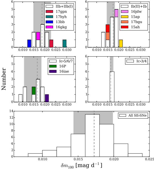
Figure 12. (top) The distribution of late time decay rates for SE-SNe; the median is \sim 0.017 mag \text{d}^{-1} for all SN types. Only SN 2013bb has had host-galaxy flux subtracted, but the effect of this on \delta m_{100} was found to be negligible at this phase, \sim 0.001 mag \text{d}^{-1} . The dashed line and grey regions are as in Fig. 9.
