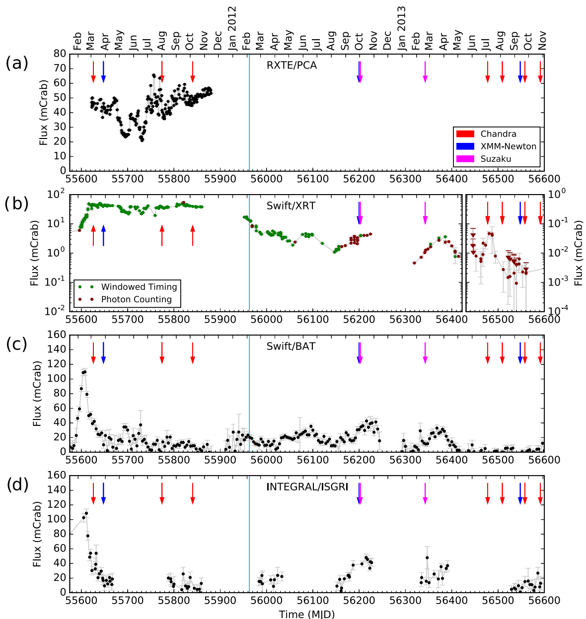
Figure 2. RXTE (panel a), Swift /XRT (panel b), Swift /BAT (panel c) and INTEGRAL /IBIS (panel d) light curves of IGR J17091–3624 during its 2011–2013 outburst. Arrows mark times at which XMM-Newton (blue), Chandra (red) or Suzaku (magenta) observed IGR J17091–3624. The cyan line represents MJD 55963, the approximate time IGR J17091–3624 transitions from the soft to the hard state (Drave et al. 2012). RXTE /PCA (Jahoda et al. 1996) data are for the 2–16 keV energy band and taken from Altamirano et al. (2011a), Swift /BAT (Barthelmy 2000) data are for 15–50 keV, Swift /XRT (Burrows et al. 2003) data are for 0.3–10 keV and INTEGRAL /ISGRI (Ubertini et al. 2003) data are for 20–40 keV. Note that the data from Swift /XRT (panel b) are shown with a logarithmic y-axis to better show the late-time progression of the outburst. Data points are coloured according to the observing mode used. The Swift /XRT data from times later than MJD 56422 are shown to a different scale to better represent the post-outburst evolution of the source. All data are presented in 1 d bins, except for data from Swift /BAT, which is presented in 4 d bins. See also Fig. 3, in which data from RXTE /PCA are presented on a smaller scale. The Crab count rates used to normalize these data were 2300 counts s −1 PCU −1 , 747.5 counts s −1 , 0.214 counts s −1 and 183.5 counts s −1 for RXTE , Swift /XRT, Swift /BAT and INTEGRAL /ISGRI, respectively. RXTE data have not been corrected for the 25 arcmin offset to avoid contamination from GX 349+2, and for all instruments we implicitly assume that IGR J17091 presents a Crab-like spectrum.
