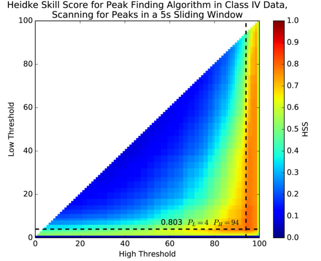
Figure A2. The Heidke skill score of a class IV observation of IGR J17091–3624 for a selection of different values P_L and P_H .
