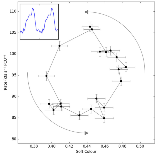
Figure 8. The HID_1 of the class III observation 96420-01-04-01, orbit 0. The data have been folded over a period of 79.61 s, corresponding to the peak frequency in the Lomb–Scargle spectrum of this observation. Inset is the folded light curve of the same data.
