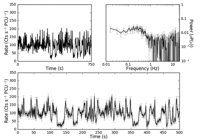
Figure 15. Plots of the class V1 observation 96420-01-09-00, orbit 0. Top left: 750 s light curve binned on 2 s to show light-curve evolution. Top right: Fourier PDS. Bottom: light curve binned on 1 s.
