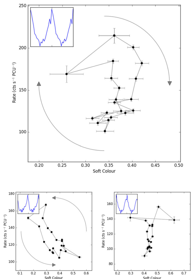
Figure 16. Top: the \text{HID}_1 of the class VI observation 96420-01-30-03, orbit 0 showing a clockwise loop. The data have been folded over a variable period found with the algorithm described in Appendix A. Inset is the folded light curve of the same data. Bottom left: the \text{HID} of class VI observation 96420-01-30-04 orbit 0, an example of an anticlockwise loop. Bottom right: the \text{HID} of class VI observation 96420-01-09-03 orbit 0, in which we were unable to ascertain the presence of a loop.
