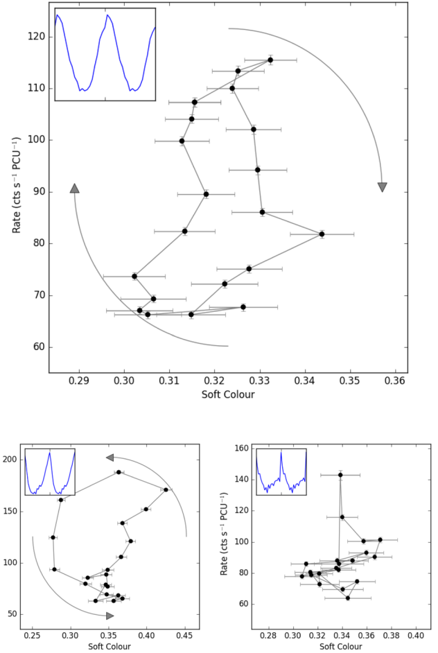
Figure 14. Top: the HID_1 of a type V_1 flaring region in class V observation 96420-01-07-00, orbit 0 showing a clockwise loop. The data have been folded over a variable period found with the algorithm described in Appendix A. Inset is the folded light curve of the same data. Bottom left: the HID_1 of class V observation 96420-01-25-05 orbit 0, an example of an anticlockwise loop. Bottom right: the HID_1 of class V observation 96420-01-25-06 orbit 0, in which we were unable to ascertain the presence of a loop.
