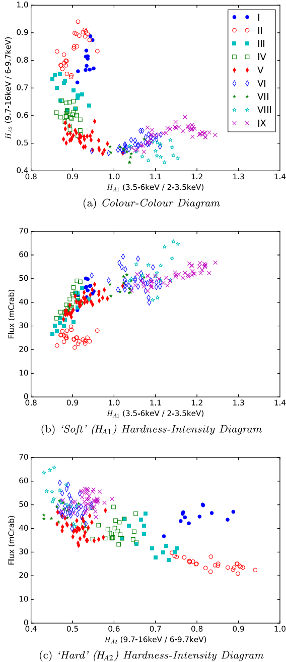
Figure 4. A global colour–colour diagram (a), ‘soft’ HID (b) and ‘hard’ HID (c) of the 2011–2013 outburst of IGR J17091, using the colours H_{A1} and H_{A2} defined previously. Observations belonging to different classes have been highlighted in different colours. Data taken from Altamirano et al. (2011a).
