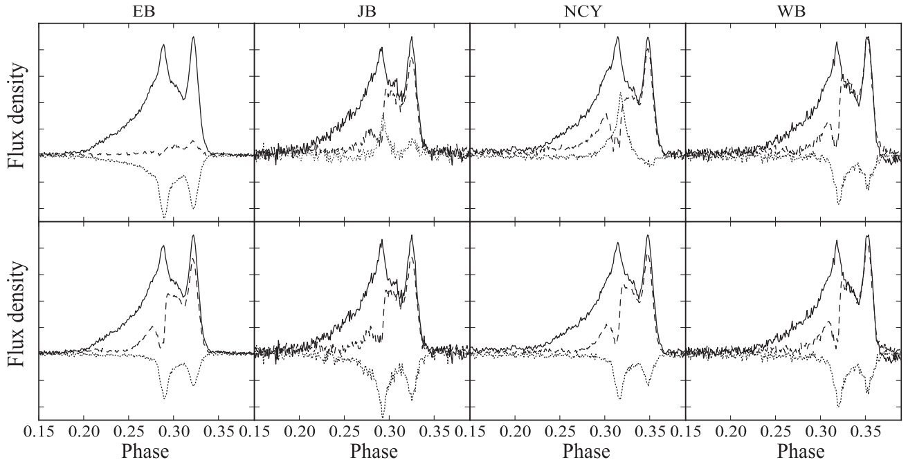
Figure 4. Pulsar profiles of PSR J1022+1001 as observed with the individual telescopes before and after polarization calibration. The solid, dashed and dotted curves are for total intensity, linear polarization and circular polarization, respectively. The top row is the profile without calibration, and the bottom row are the calibrated ones. The EB, JB, NCY and WB abbreviations indicate the Effelsberg, Jodrell, Nançay and Westerbork telescopes. Here the y-axis, flux, takes an arbitrary unit, and x-axis is pulse phase. The calibrated profiles clearly show much better consistency.
