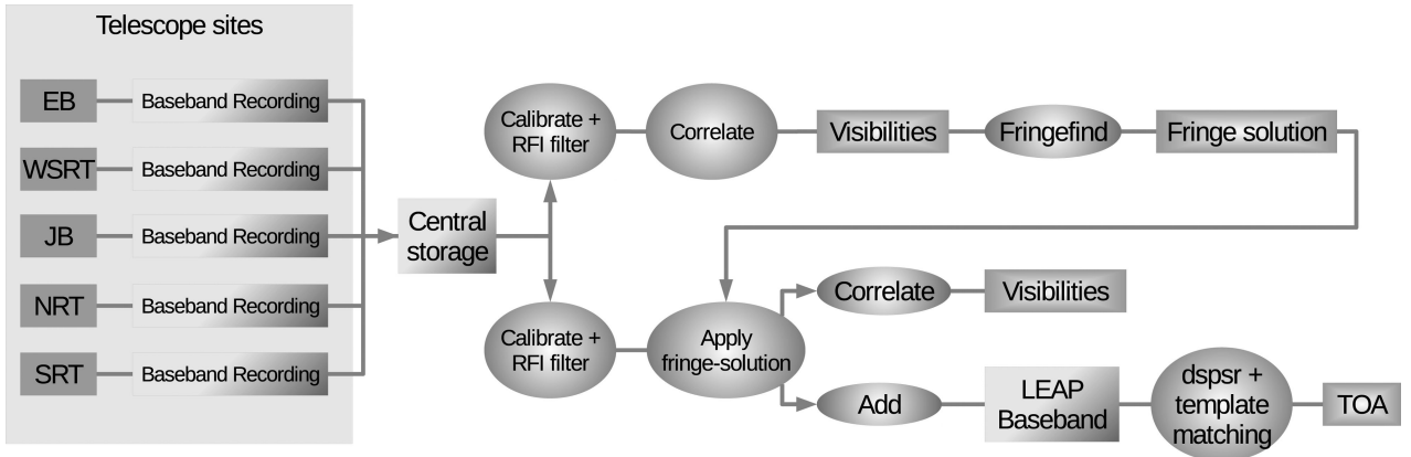
Figure 1. A flowchart of the LEAP data processing pipeline. Each observatory stores the baseband data from single-telescope LEAP observations on disc. The data are then transferred to the central storage machine at Jodrell Bank Observatory. There, polarization calibration and RFI mitigation filters are applied to the single-telescope data, which are then correlated, resulting into a fringe solution for each of LEAP’s baselines (10 telescope pairs in total). At this stage, we apply the fringe solution to each telescope’s baseband data (again after polarization calibration and RFI mitigation), correlate the time series again, and check the resulting ‘visibilities’ to verify that the fringe solution is indeed correct. The baseband data (to which the fringe solution is applied) are then added together in phase, forming the LEAP tied array. The added baseband data are processed as normal timing data. The data are then dedispersed and folded (using dpsr) and template matching is performed to produce the final pulse TOAs.
