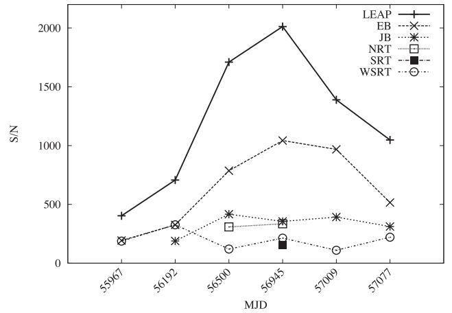
Figure 8. S/Ns from LEAP versus S/Ns from the individual telescopes for PSR J1022+1001 for the observations where coherent addition could be performed. The earliest observation shown is from 2012 February, the last observation shown is from 2015 February. The graph shows that the LEAP data provide the expected improvement in S/N, meaning that the sum of the S/Ns of the individual telescopes is roughly identical to the S/N of LEAP.
