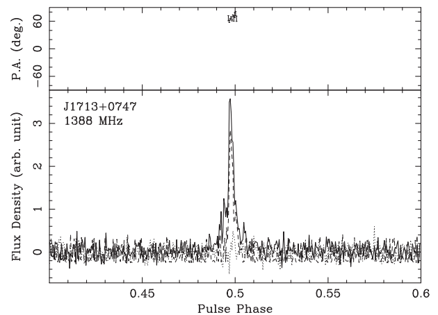
Figure 12. Polarization profile of a single pulse from PSR J1713+0747, obtained from the observation used in Fig. 11.
