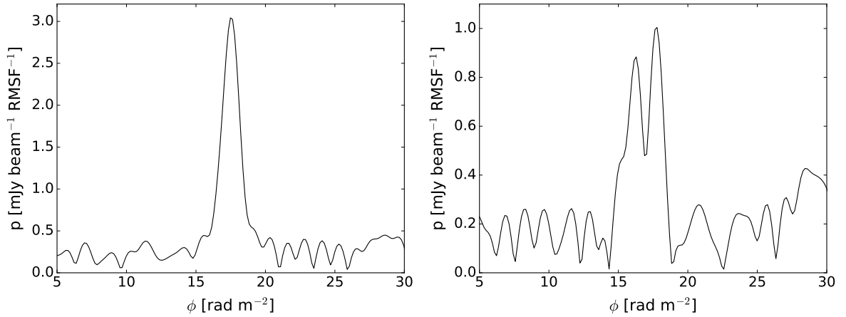
Figure 6. Example FDFs from the blazar ILT J141945.53+542314.4 (shown in Figure 4, bottom right). Left panel: Simple FDF of the blazar core with a polarised intensity of \sim 3 mJy beam ^{-1} at a Faraday depth of 17.5 rad m ^{-2} . Right panel: Complex FDF of the western extension of the blazar, with a peak of \sim 1.0 mJy beam ^{-1} at 17.7 rad m ^{-2} and a second peak of \sim 0.88 mJy beam ^{-1} at 16.2 rad m ^{-2} .
