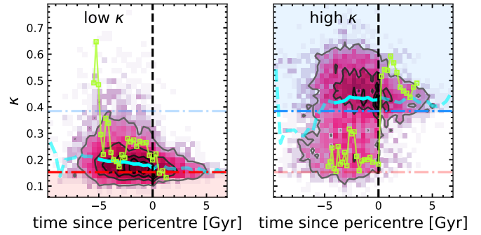
Fig. 4. Evolution of the fraction of co-rotational energy as a function of the time since the pericentre passage for low (left) and high (right) \kappa sub-sample as classified by the 5th and 95th percentiles of the z = 0 \kappa distribution in Fig. 2. Contours show 75, 50, 25, and 5% of the maximum counts of the 2D distribution. The cyan solid line shows the median value at each time bin. For bins in which less than 50% of the sample entered the median calculation, we instead use a dashed line. The red and blue horizontal dash-dotted lines show the \kappa threshold values for the low and high \kappa sub-samples, respectively. The pericentre is marked with a vertical dashed line. In each panel we additionally show the evolution of a galaxy from the corresponding sub-sample using green square markers. The shaded red and blue regions show the allowed \kappa values corresponding to each sub-sample.
