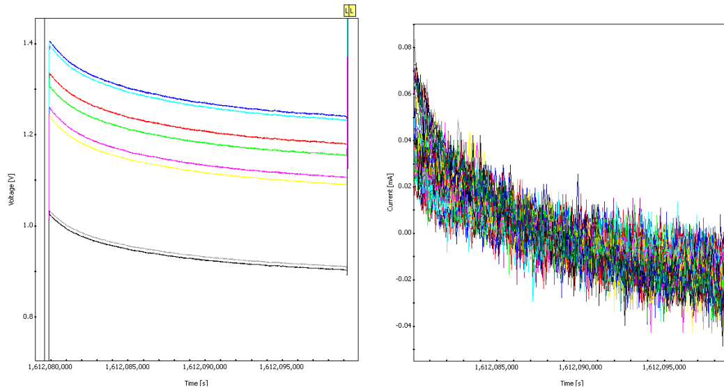
Figure 20 Signal drift (RCA 27 ) and Id overall drift )(all channels) due to thermalization.
