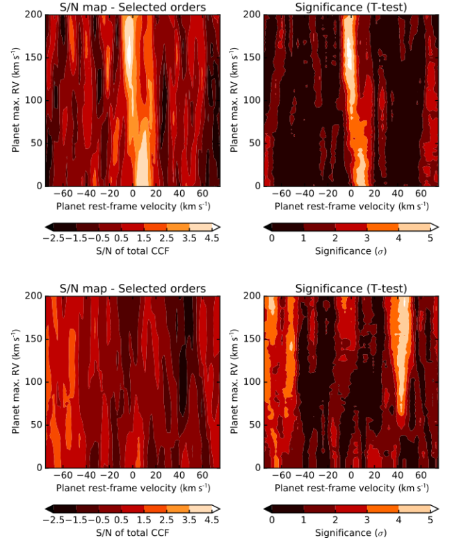
Fig. 5. Detection of H 2 O in the transmission spectrum of HD 189 733 b observed on July 11, 2015 ( top panels ) and the non detection on the night of July 30, 2015 ( bottom panels ). The total cross-correlation signal is shown as function of rest-frame velocity v_{\text{rest}} and planet radial velocity semi-amplitude K_p . The measured S/N and corresponding significances are shown in the left and right panels , respectively. These are computed as explained in Sect. 3.3. The cross-correlation shown here is obtained with a model spectrum containing H 2 O at VMR = 10 -4 and CH 4 at VMR = 10 -12 .
