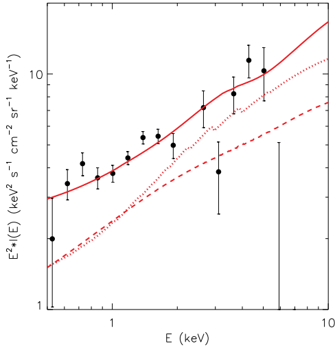
Figure 5. The spectrum of the uCXB (circles) as measured with Chandra ACIS-I in this work. The uCXB spectrum is compared with AGN synthesis models by Treister et al. (2009) (red dotted line), Gilli et al. (2007) (red continuous line) and Ballantyne et al. (2011) (red dashed line) after the survey X-ray selection function is applied (galactic N_H correction is irrelevant).
