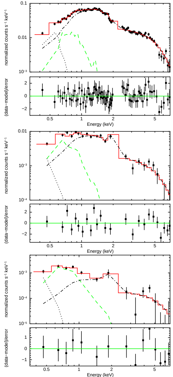
Figure 2. From top to bottom the binned CXB, uCXB and nsCXB folded spectra, respectively. Black squares are the data points. The red continuous line is the best fit model, the dot-dashed-line is the extragalactic components, the green-dashed line is the hard thermal component and the dotted line is the local bubble components. In the bottom panels we show the fit residuals. Data have been re-binned in order to have at least 10\sigma significance per bin and no more than 20 bins have been combined.
