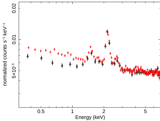
Figure 1. A comparison of the nsCXB (red stars) before background subtraction and the PIB (black triangles). It is worth to note that the error bars of the PIB spectrum are much larger than those of the raw nsCXB spectrum.
