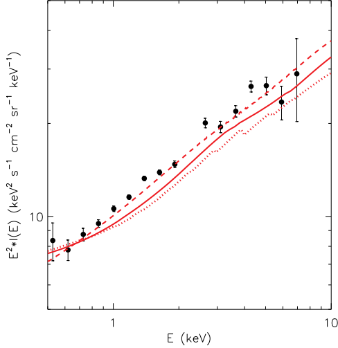
Figure 4. The unfolded CXB spectrum measured by Chandra with ACIS-I (black) in this work. Overplotted to the data we show AGN population synthesis models, after adding cluster emission (Gilli et al. 1999), and star forming galaxies emission (Cappelluti et al. 2016), by Treister et al. (2009) (red dotted line), Gilli et al. (2007) (red continuous line) and Ballantyne et al. (2011) (red dashed line). The extragalactic CXB spectrum is well fitted by a power-law model with photon index \Gamma \sim 1.45 and normalization \sim 10.91 \text{keV cm}^2 \text{s}^{-1} \text{sr}^{-1} .
