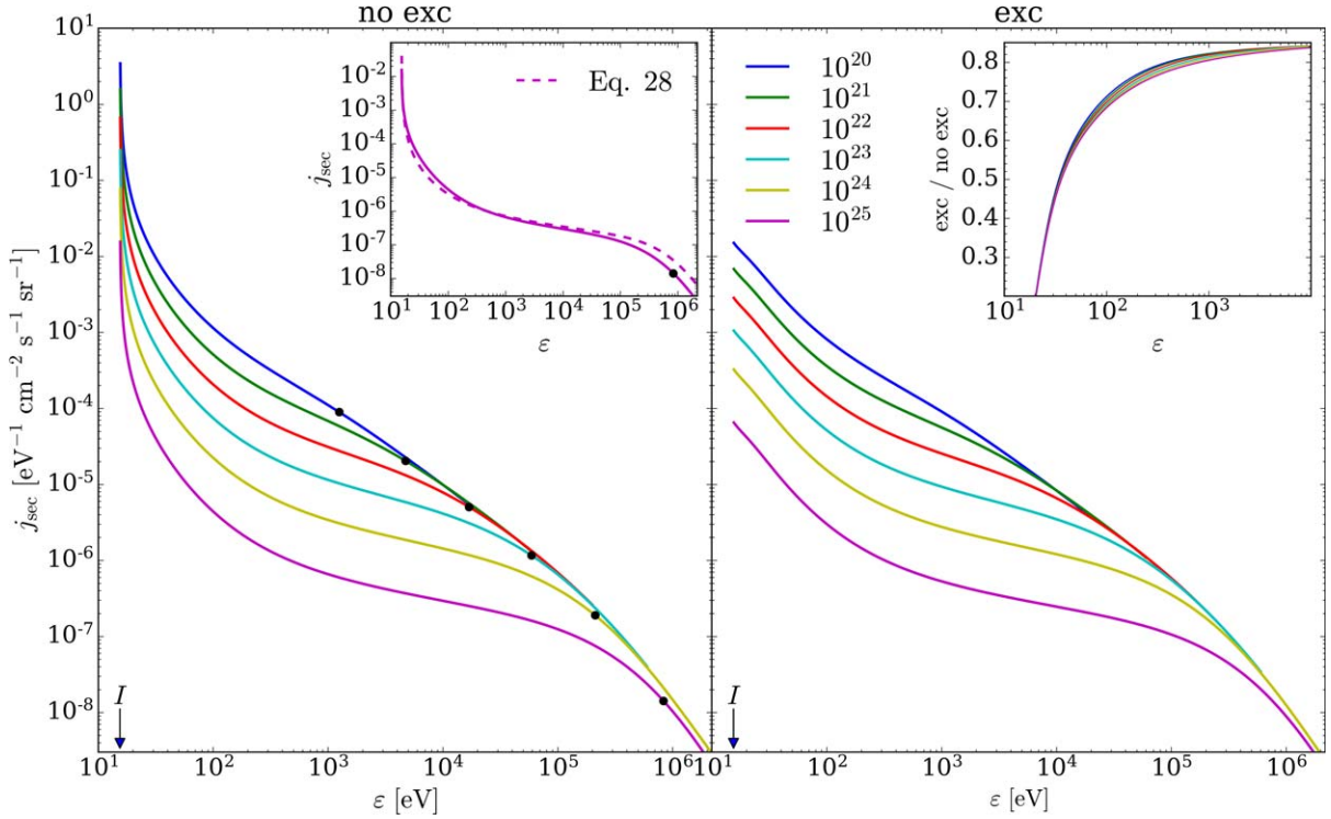
Figure 2. Energy spectra of secondary electrons j_{\text{sec}}(\epsilon) obtained for the interstellar proton spectrum \mathcal{H} from a numerical solution of Equation (27) for different N (see the legend, in units of \text{cm}^{-2} ). The vertical arrows in the bottom left corners of the panels indicate where \epsilon = I . The left panel shows the spectra for a model case where excitation collisions are omitted; agreement between the numerically computed spectrum and the high-energy analytical asymptote, Equation (28), is illustrated for N = 10^{25} \text{ cm}^{-2} in the inset. The bullets for different curves indicate where \epsilon = \epsilon_{\text{att}}(N) . The right panel displays the results with excitation; the inset shows these spectra normalized by j_{\text{sec}}(\epsilon) that are plotted in the left panel.
