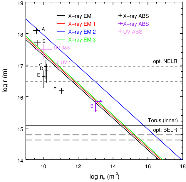
Fig. 7. Distance and number density of optical, UV and X-ray emission and/or absorption components in NGC 5548. The solid diagonal lines are the distance and density relations (i.e. \log \xi = L/n_H r^2 ) of the X-ray emission components (EM for Whewell et al. 2015, and EM 1–3 for Model T). The black pluses ( 1\sigma uncertainties) refer to the six warm absorber components (via a timing analysis, Ebrero et al. 2016). The purple arrows are the 3\sigma upper (distance) and lower (density) limits of the warm absorber component B (via a spectral analysis, Mao et al. 2017). The pink pluses are for the UV absorption components (Arav et al. 2015). The horizontal short dashed lines refer to the optical narrow emission line region (Peterson et al. 2013). The horizontal long dashed lines refer to the optical broad emission line region (Kaspi et al. 2000; Bottorff et al. 2002). The horizontal dotted line indicates the inner edge of the torus (Suganuma et al. 2006).
