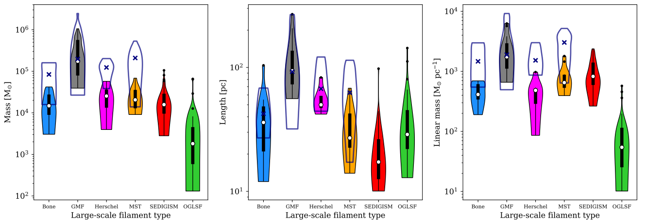
Fig. 3. Violin- (colours) and box-plot (black) representations of the distributions of mass (left), length (middle), and linear mass (right) of Galactic LSFs. Following Zucker et al. (2018) , IGLSFs are divided into Milky Way ‘bones’ (blue), GMFs (grey), Herschel filaments (magenta), minimum spanning tree (MST) filaments (yellow). IGLSFs identified from the Structure, Excitation, and Dynamics of the Inner Galactic InterStellar Medium (SEDIGISM, Schuller et al. 2017 ) survey data are in red (from Mattern et al. 2018b ). OGLSFs, observed within our data, are in green. More information on IGLSFs are reported in Appendix B.2. The white circles show the median for each property and sub-sample. For comparison, the transparent violins show the measurements of Zhang et al. (2019) for the same category of structures, where the ‘x’ indicates the median of the samples.
