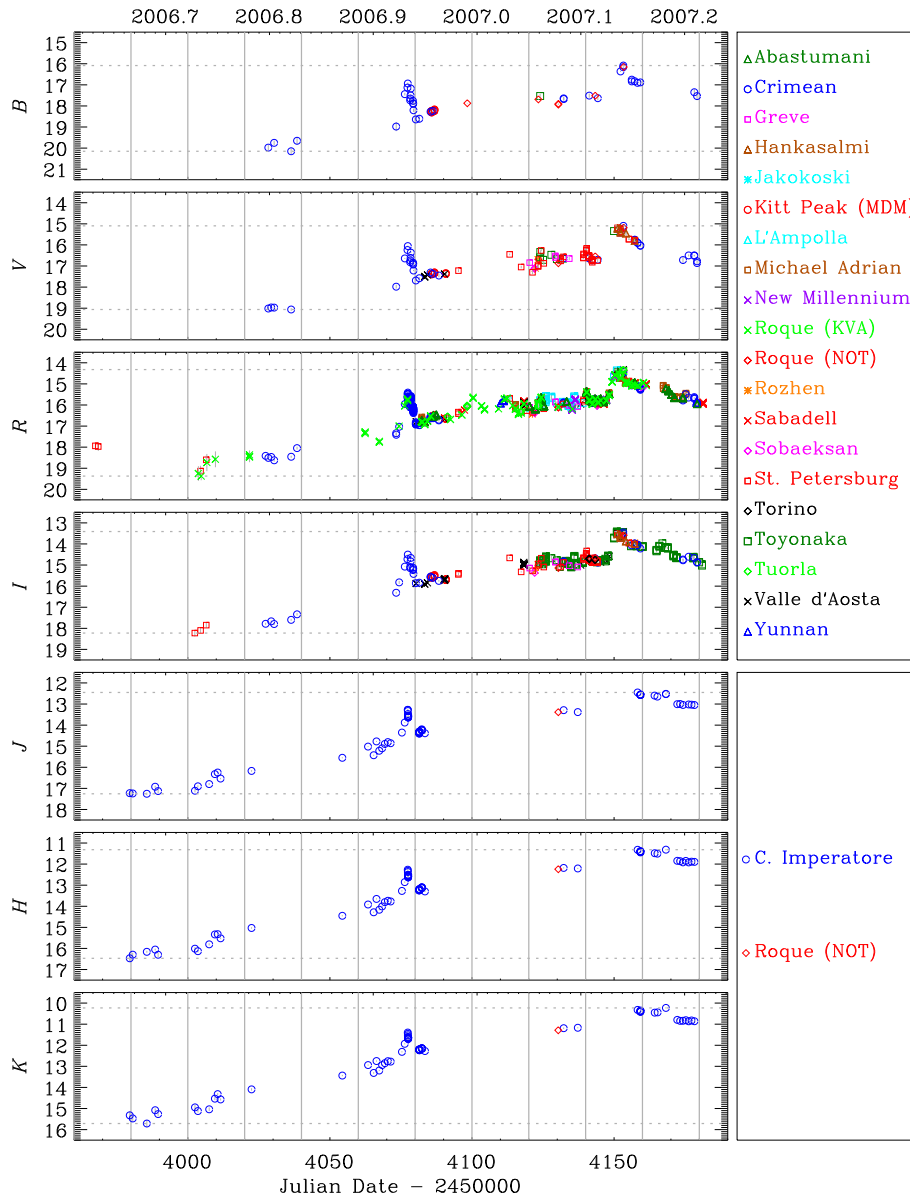
Fig. 1. Optical and near-IR light curves of AO 0235+164 in the 2006–2007 observing season. The optical magnitudes are corrected for the ELISA contribution. Maximum and minimum brightness levels are highlighted with horizontal dotted lines.
