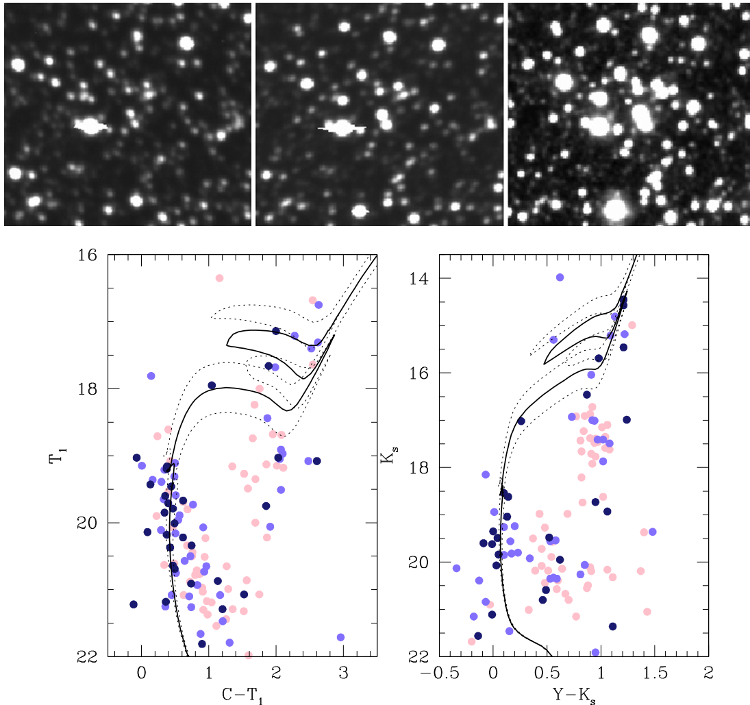
Figure 3. Top: C , T_1 and K_s images (from left to right) centred on the new star cluster candidate VMC17. The images' sides are equal to the star cluster diameter (see Table 1). North is up and East to the left. Bottom: Washington and VMC CMDs illustrating the performance of the cleaning procedure, where we plotted all the measured stars located within the cluster radius. The pink, light and dark blue filled circles in the bottom panels represent stars with cluster membership probabilities P \leq 25 per cent, P = 50 per cent, and P \geq 75 per cent, respectively. Three isochrones from Bressan et al. (2012) for \log(t \text{ yr}^{-1}) = 8.3, 8.4 , and 8.5 and Z = 0.003 are also superimposed.
