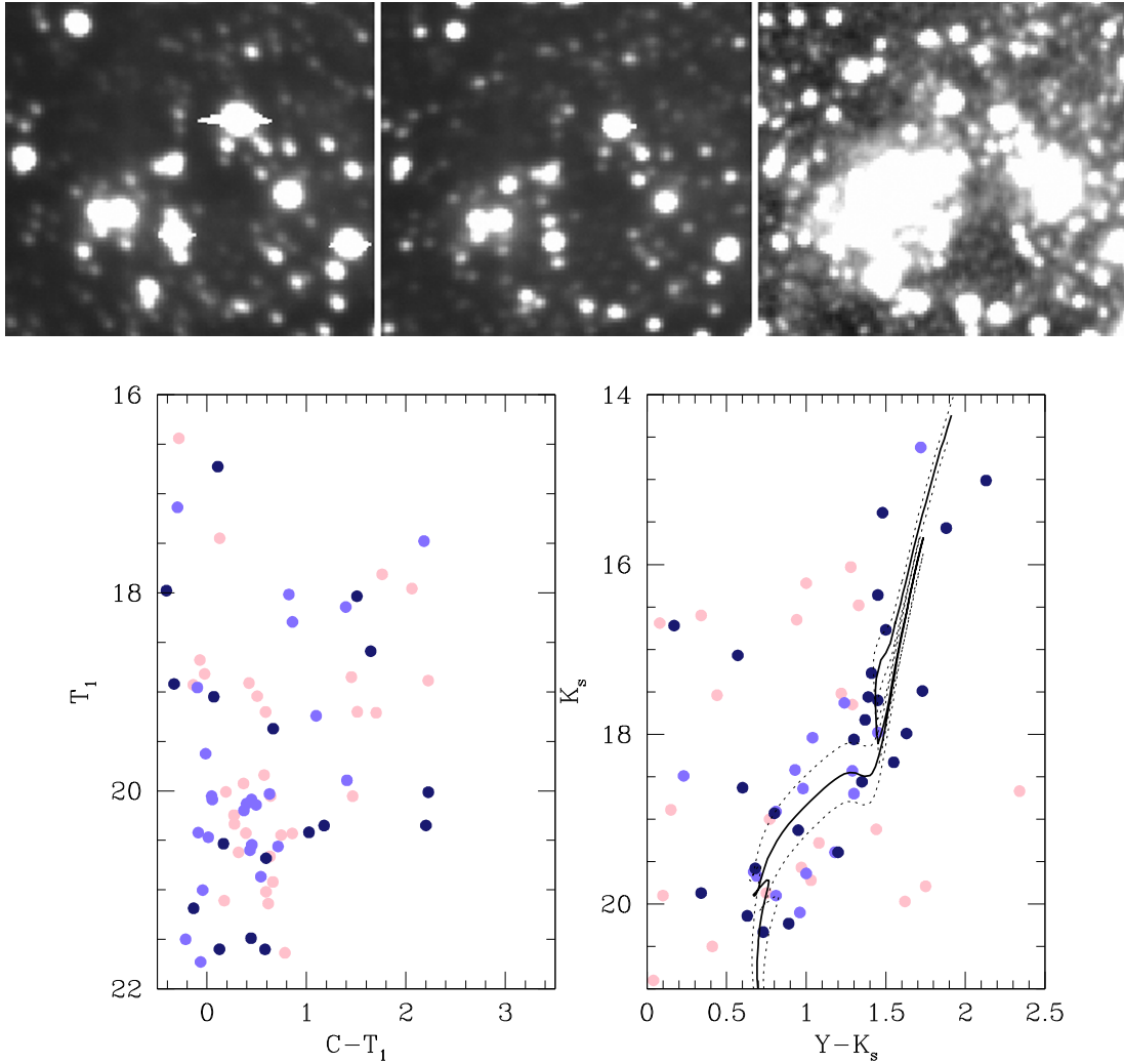
Figure 4. Same as Fig. 3 for the new star cluster candidate VMC9. Three isochrones from Bressan et al. (2012) for \log(t \text{ yr}^{-1}) = 8.9, 9.0 , and 9.1 and Z = 0.003 are also superimposed.
