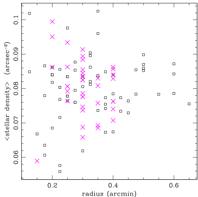
Figure 2. Relationship between the stellar density and the cluster radius in the studied SMC field. The typical background stellar density ranges between 0.008 and 0.012 arcsec -2 . Open black squares and magenta crosses represent previously catalogued and new star cluster candidates, respectively.
