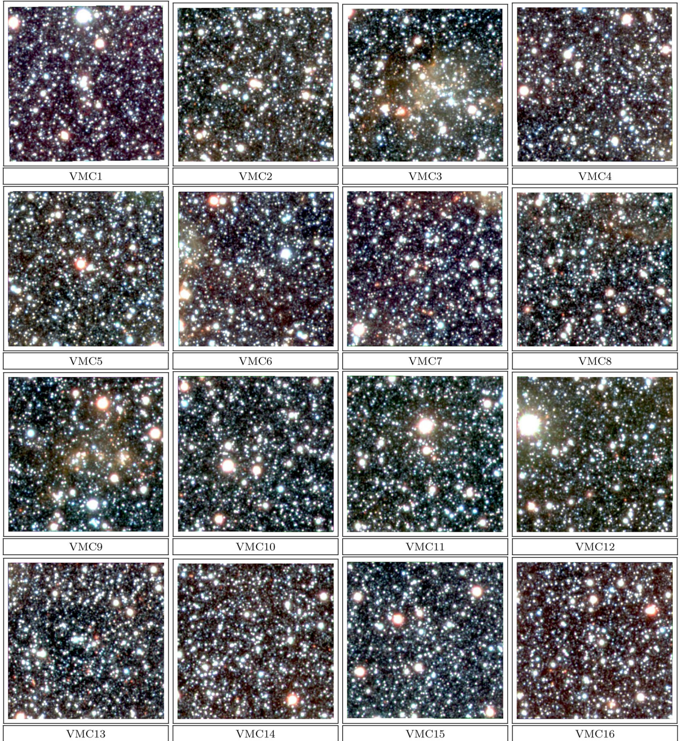
Figure A1. 2 \times 2 arcmin 2 YJK_s images centred on the new SMC star clusters. North is up and East to the left. Note that the star clusters' radii are between 0.15 and 0.40 arcmin.
