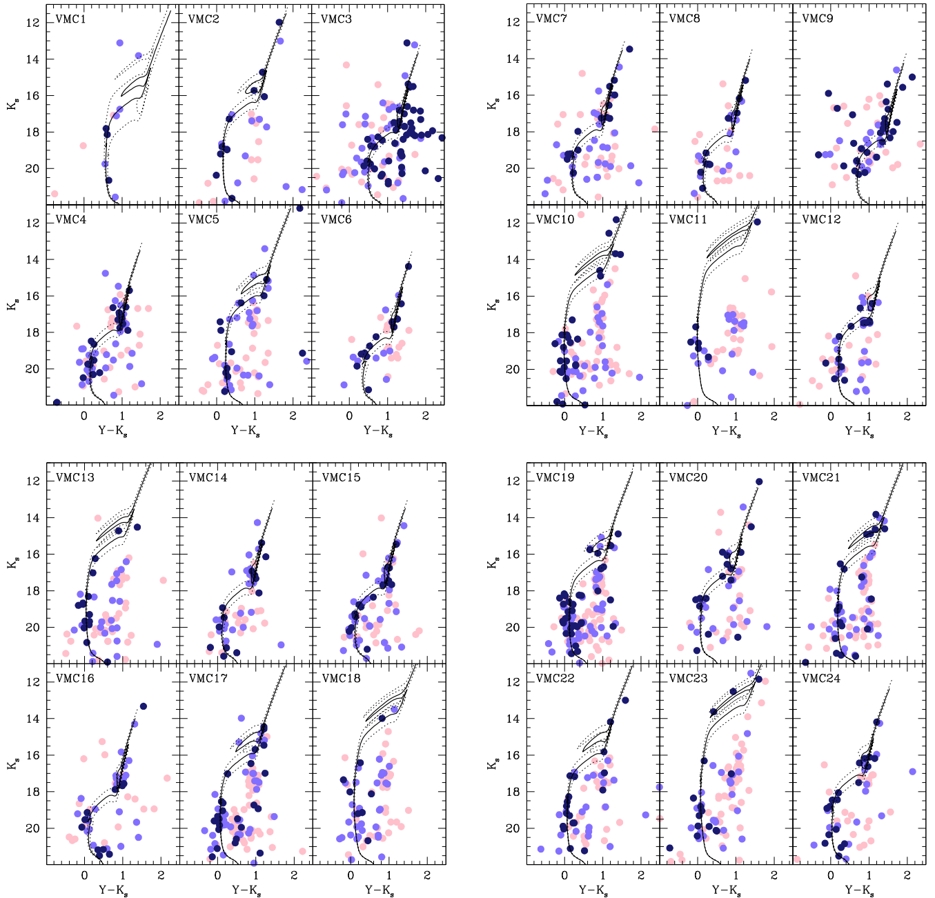
Figure A2. K_s versus Y - K_s CMD of stars within the cluster radius. Colour-coded symbols represent stars that statistically belong to the field ( P \leq 25 per cent, pink), stars that might belong to either the field or the cluster ( P = 50 per cent, light blue), and stars that predominantly populate the cluster region ( P \geq 75 per cent, dark blue). Three isochrones from Bressan et al. (2012) for \log(t \text{ yr}^{-1}) and \log(t \text{ yr}^{-1}) \pm 0.1 are also superimposed.
