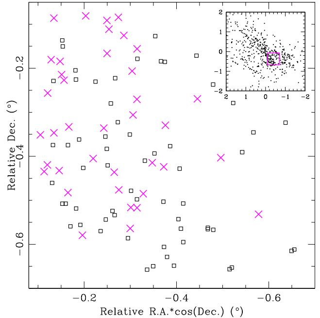
Figure 1. Pilot region chosen to search for new star clusters. Open black squares and magenta crosses represent previously catalogued and new star clusters, respectively. The inset panel depicts the spatial distribution of the catalogued SMC star clusters. A thick magenta-coloured open box delimits the studied SMC field. We used as the SMC centre: RA = 00h 52m 45s, Dec = -72^\circ 49' 43'' (J2000) (Crowl et al. 2001).
