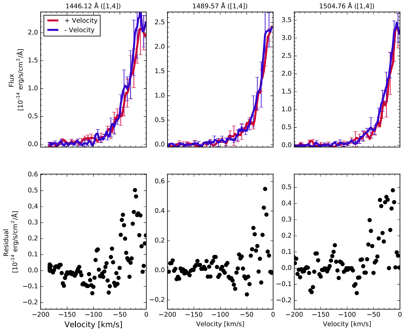
Figure 10. Mirrored profiles of \text{H}_2 emission lines from the [1, 4] progression. An Anderson–Darling test was conducted for each feature to determine whether differences between the red and blue sides of the line profiles are statistically significant ( p < 0.05 ). At the resolution of our data, there are no meaningful asymmetries.
