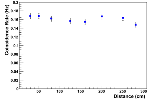
Fig. 9. Coincidence rate between one of the scintillator strips and an external trigger scintillator, as a function of its distance with respect to the photosensor.
