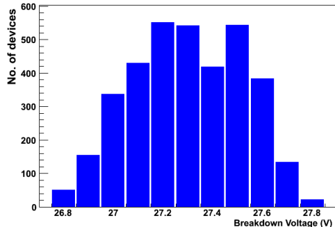
Fig. 4. Breakdown voltage distribution, measured over a sample of about 4500 devices.
