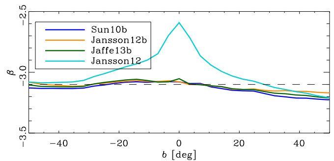
Fig. 8. Effective synchrotron spectral index, \beta , between models at 30 GHz and the data at 408 MHz as averaged over latitude bins in the inner Galaxy ( -90^\circ \leq l \leq 90^\circ ).
