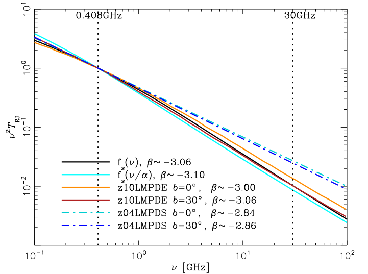
Fig. 2. Comparison of synchrotron spectra for different CRL models, all normalized to one at 408 MHz. The black solid curve shows the original spectral template used in the Commander analysis, while the cyan solid curve shows the shifted template as described in Planck Collaboration X (2016). In orange is the resulting SED on the plane for synchrotron emission computed using the z10LMPDE CRL model on which the Commander template is based. This curve shows the average curve for the Galactic plane, while the brick red is the average for the pixels on a ring at b = 30^\circ . For these spectra, the effective spectral index \beta = \log(A_{30}/A_{0.408})/\log(30/0.408) is computed. Lastly, the light and dark blue dot-dashed lines show the power law with the effective indices for the z04LMPDS model averaged at the two latitudes.
