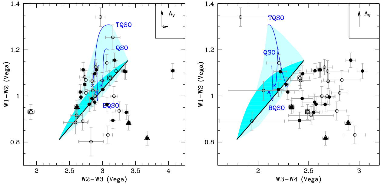
Figure 2. The expected positions on the W1 - W2 versus W2 - W3 (left) and W1 - W2 versus W3 - W4 (right) plot of AGNs with different shapes of IR spectrum: (1) a simple power law (PL; black thick line) with slope ranging from 0.5 to 1.5; (2) a smooth broken PL, with slope before the break ranging from 0.5 to 1 and a slope of 1.5 after the break and with the break position varying within the WISE bands (dark blue shaded area); (3) an RQ AGN emission described by the three QSO templates from the SWIRE library (blue lines labelled as QSO, BQSO and TQSO, see text for a description and Polletta et al. 2007 for more details) and with a redshift ranging from 0 (indicated by a cross) to 0.9 (the maximum value of the sample); (4) a combination of RQ AGN emission plus a PL spectrum (light blue shaded area). In particular, we show the result of all the different combinations of slopes (from 0.5 to 1.5), redshift (from 0 to 0.9) and relative RQ AGN to PL normalization. The arrows in the upper-right corners show the expected effect of an extinction of A_V = 2 mag at the mean redshift of the sample. An A_V = 2 mag is the maximum value expected for type 1 AGNs. We do not plot the arrow along the W3 - W4 since the extinction has a negligible effect in this case. Points as in Fig. 1.
