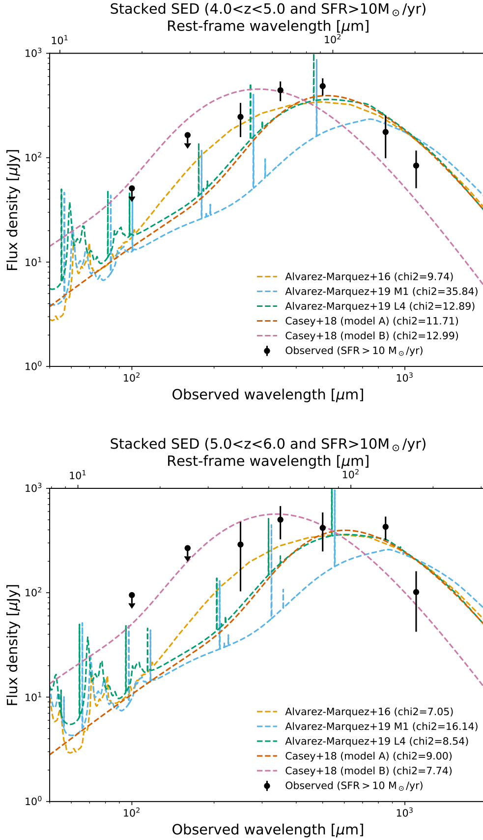
Fig. A.3. Comparison of the discarded dust SED templates with the stacks of Herschel data at z \sim 4.5 and z \sim 5.5 . The black symbols are stacked Herschel data and the dashed lines are templates from the literature.
