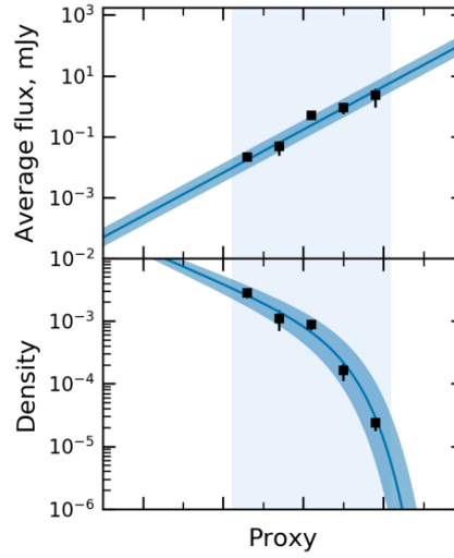
Fig. 2. Illustration of the method used to determine the \text{SFRD}_{\text{IR}} . Left panel: steps performed. Right panel: arbitrary proxy density function (UVLF or GSMF) and a power law relation between the property used as a proxy and the FIR flux. The black squares represent measured values and the solid line the fit with uncertainties represented by a shaded region. The vertical shaded regions show the proxy range, in which the data is available for both the power law relation derived from ALPINE and the proxy density function.
