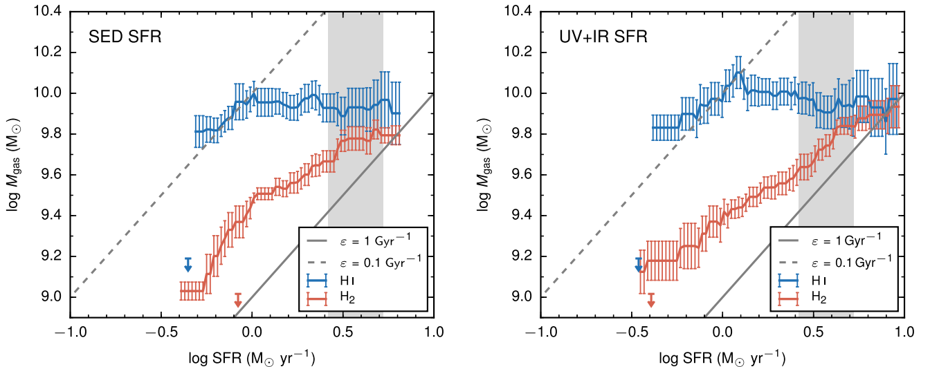
Figure 6. Average atomic gas mass (in blue) and molecular gas mass (in red) as a function of SFR for central disk galaxies in the stellar mass range of 10^{10.6} – 10^{11} M_\odot , plotted by using two different SFR estimates. The SFRs used in the left panel are derived from the SED fitting of UV, optical, and mid-IR bands (Salim et al. 2018). The SFRs used in the right panel are given by the xCOLD GASS catalog (Saintonge et al. 2017) and they are derived from the near-UV and mid-IR photometries by the technique described in Janowiecki et al. (2017). All labels in this plot are the same as those in Figure 4.
