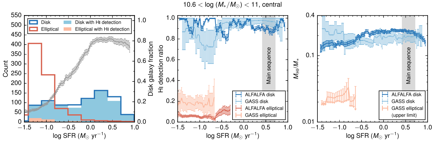
Figure 2. Left: SFR distribution function for central disk galaxies (blue line) and central elliptical galaxies (red line) in the narrow stellar mass range of 10^{10.6} - 10^{11} M_{\odot} . The shaded regions show the SFR distribution of galaxies with H I detection, in blue for central disks and in red for central ellipticals. About 30% of the galaxies with uncertain morphology are not shown here. The gray line shows the fractional abundance of disk galaxies, obtained by using a sliding average of 0.5 dex in SFR. Error bars are derived from the binomial error of the fraction with 68% confidence level. Middle: H I detection ratio in ALFALFA and GASS as a function of SFR for central disk galaxies (blue lines) and central elliptical galaxies (red lines) in the stellar mass range of 10^{10.6} - 10^{11} M_{\odot} . These values are determined by using the sliding average of 0.5 dex in SFR, and error bars are derived from the binomial error of the fraction with 68% confidence level. Right: H I gas mass to stellar mass ratio ( M_{\text{HI}}/M_* ) for central disk galaxies and central elliptical galaxies (upper limit) in the same stellar mass range. For elliptical galaxies in GASS, the upper limits of nondetections are included in the average so that it is plotted as pink arrows. The error bars on the lines indicate the 1\sigma uncertainty around the mean value. The gray shades indicate the position of the star-forming main sequence defined in Renzini & Peng (2015).
