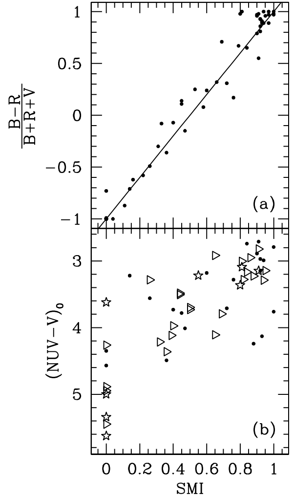
Fig. 3. Panel a ): correlation of the SMI with the HBR index ( \frac{B-R}{B+R+V} ) for our sample of Galactic GCs. HBR values are taken from the latest version of the Harris (1996) catalogue. The continuous line is the relation between \frac{B}{B+R} and \frac{B-R}{B+R+V} from Preston et al. (1991), reported in Eq. (1). Panel b ): correlation of SMI with the integrated ultraviolet-optical color (NUV - V)_0 for Sample A (open stars), Sample B (open triangles, to be considered as lower limits), and Galactic GCs (small filled circles).
