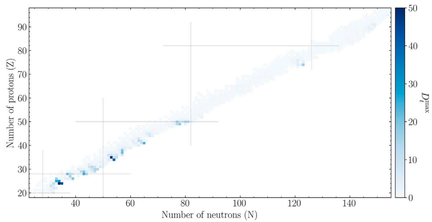
FIGURE 6 Nuclear heating rate sensitivity across the nuclear chart. For each nucleus, the shading represents the maximum sensitivity measure D_t attained at any time t = 0.1, 1, 10, 100 days.
