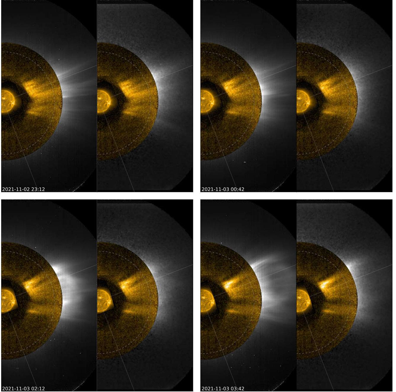
Fig. 8. Propagation of a CME across the FSI and Metis FOVs. Left and right sides of each panel show a comparison of SWAP (below 2 R_{\odot} ) and FSI 17.4 nm (up to 5.6 R_{\odot} ) with Metis VL and Lyman \alpha data, respectively. The dashed circle marks the position of the edge of the Metis occulting disk. An animated version of the figure is available online .
