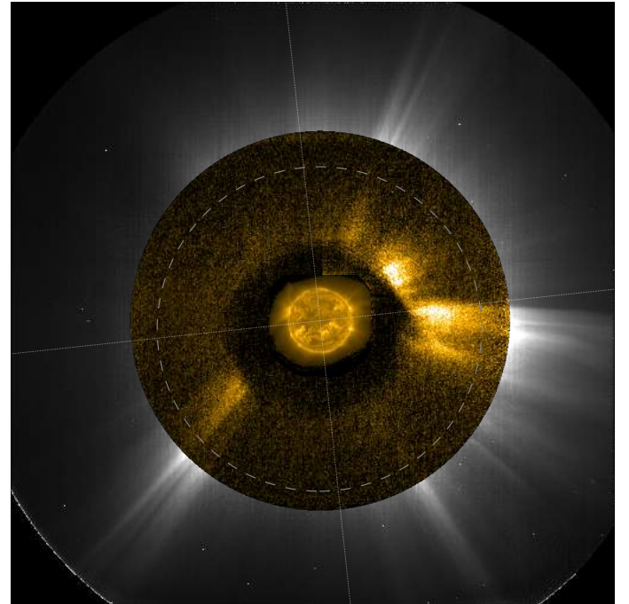
Fig. 12. Composite of images taken on 2022 December 15: EUVI-A (below 1.9 R_{\odot} , 18:34 UT), FSI 17.4 nm (below 6.1 R_{\odot} , 18:30 UT) and Metis VL (18:30 UT). The dashed circle marks the position of the edge of the Metis occulting disk. An animated version of this figure is available online .
