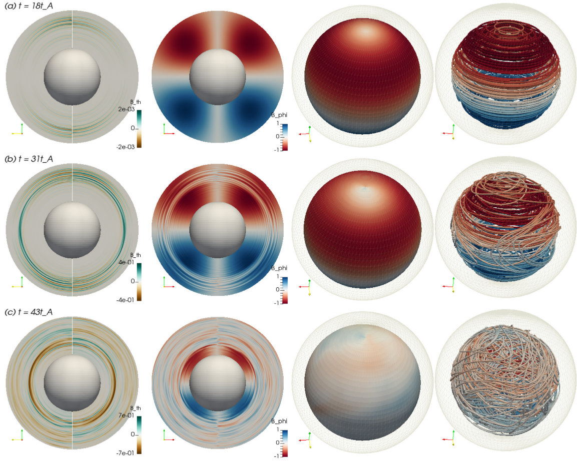
Figure 4. Same as Fig. 3, but for simulation TiA05 at t = 18t_A , 31t_A , and 43t_A . In this case, the field configurations in third and fourth columns are shown at r = 0.85R_s .
