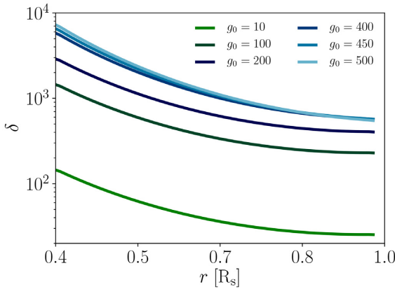
Figure 2. Radial profile of \delta for simulations TiA04, TiA07, TiA09, TiA12, TiA13, and TiA14. These simulations start with the same initial magnetic field, B_0 = 1 \text{ T} , but have different gravity at the bottom of the domain, g_0 .
