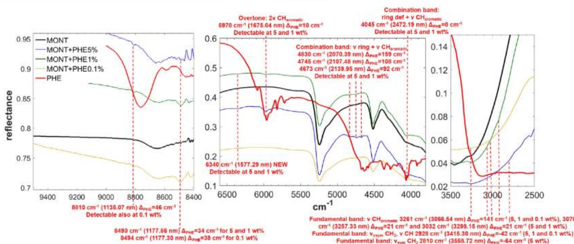
FIGURE 5 | NIR spectra of PHE adsorbed on montmorillonite at 5, 1, and 0.1 wt% concentration. Legend: \Delta_{\text{PHE}} = wavenumber shift with respect to the same peak of the pure molecule in the solid state; \nu = stretching vibrational mode; \delta = bending vibrational mode; def = deformation vibrational mode; sym = symmetric vibrational mode; asym = asymmetric vibrational mode.
