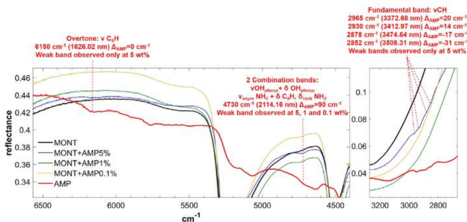
FIGURE 3 | NIR spectra of AMP adsorbed on montmorillonite at 5, 1, and 0.1 wt% concentration. Legend: \Delta_{AMP} = wavenumber shift with respect to the same peak of the pure molecule in the solid state; phosp = phosphate group; \nu = stretching vibrational mode; \delta = bending vibrational mode; rock = rocking in-plane vibrational mode; asym = asymmetric vibrational mode.
