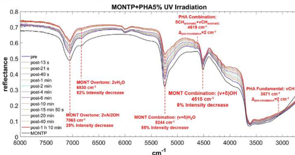
FIGURE 11 | Main changes in NIR features after 70 min of UV irradiation for PHA 5 wt% on montmorillonite containing 1 wt% of Mg-perchlorate. Legend: \Delta_{\text{pre-irr}} = wavenumber shift with respect to the same peak pre-irradiation; \nu = stretching vibrational mode; \delta = bending vibrational mode.
