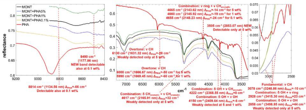
FIGURE 6 | NIR spectra of PHA adsorbed on montmorillonite at 5, 1, and 0.1 wt% concentration. Legend: \Delta_{\text{PHA}} = wavenumber shift with respect to the same peak of the pure molecule in the solid state; \nu = stretching vibrational mode; \delta = bending vibrational mode.
