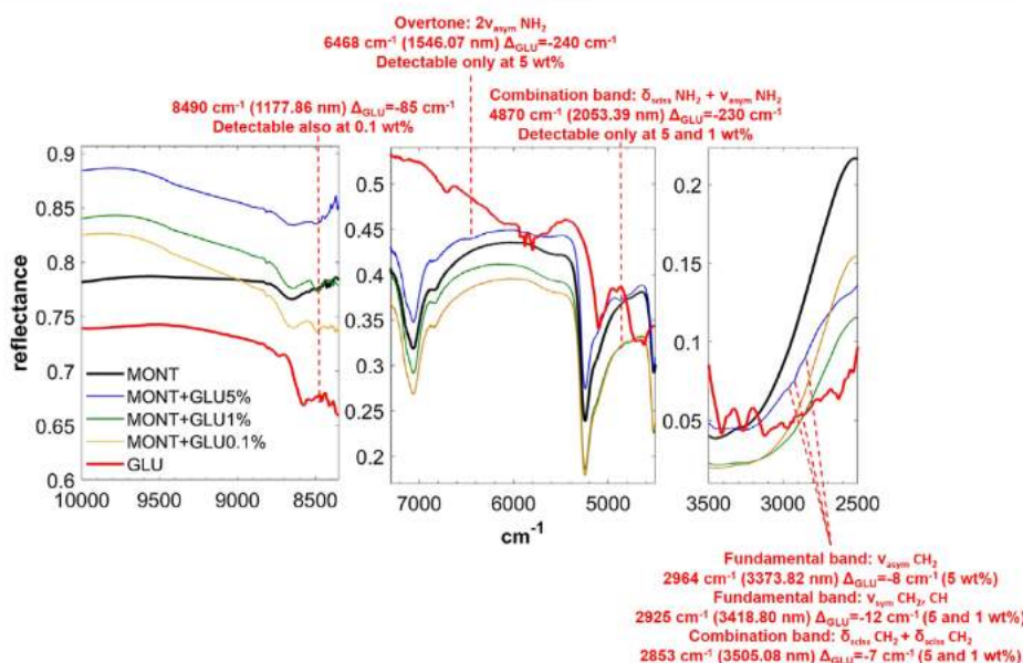
FIGURE 4 | NIR spectra of GLU adsorbed on montmorillonite at 5, 1, and 0.1 wt% concentration. Legend: \Delta_{\text{GLU}} = wavenumber shift with respect to the same peak of the pure molecule in the solid state; \nu = stretching vibrational mode; \delta = bending vibrational mode; sciss = scissoring in-plane vibrational mode; sym = symmetric vibrational mode; asym = asymmetric vibrational mode.
