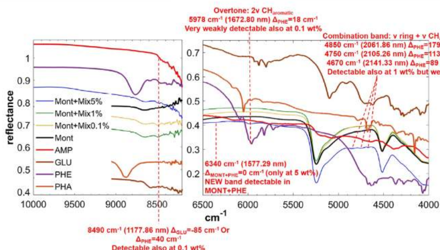
FIGURE 7 | NIR spectra of MIX adsorbed on montmorillonite at 5, 1, and 0.1 wt% concentration. Legend: \Delta_{PHE} = wavenumber shift with respect to the same peak of the pure molecule in the solid state; \Delta_{MONT+PHE} = wavenumber shift with respect to the same peak of PHE adsorbed on MONT; \nu = stretching vibrational mode.
