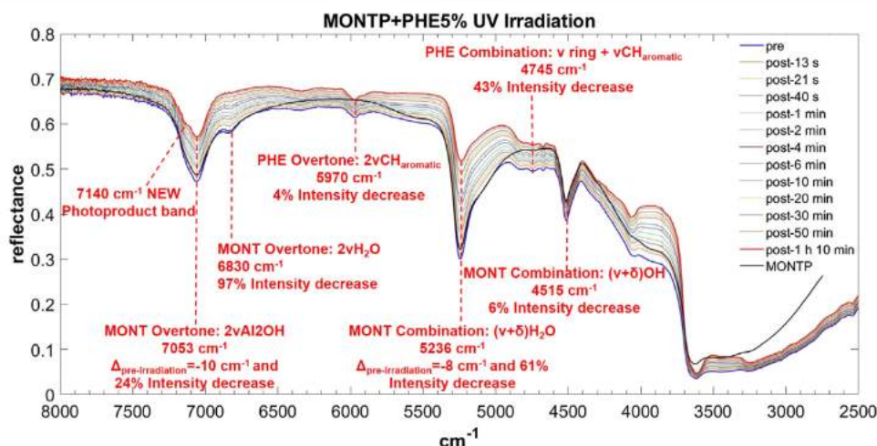
FIGURE 10 | Main changes in NIR features after 70 min of UV irradiation for PHE 5 wt% on montmorillonite containing 1 wt% of Mg-perchlorate. Legend: \Delta_{\text{pre-irr}} = wavenumber shift with respect to the same peak pre-irradiation; \nu = stretching vibrational mode; \delta = bending vibrational mode.
