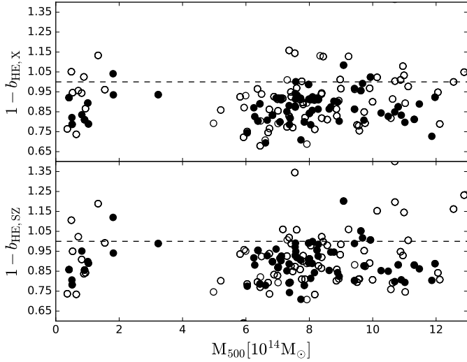
Fig. A.1. Hydrostatic mass bias vs. the cluster mass at R_{500} . Top panel: X-ray mass bias, (1 - b_{\text{HE},X}) . Bottom panel: SZ mass bias, (1 - b_{\text{HE},SZ}) . Similarly to Fig. 14 of the main text, well-fitted clusters are represented by filled points and poorly fitted objects by empty points.
