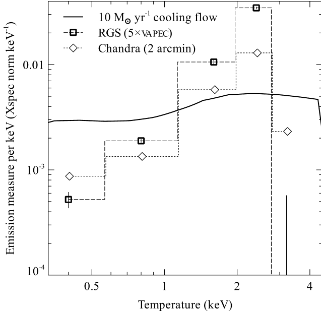
FIGURE 3 Comparison of the emission measures from RGS and Chandra observations of the Centaurus cluster core (Sanders et al., 2008). The solid line shows the expected distribution for a 10 M_{\odot} \text{ yr}^{-1} isobaric cooling flow.
