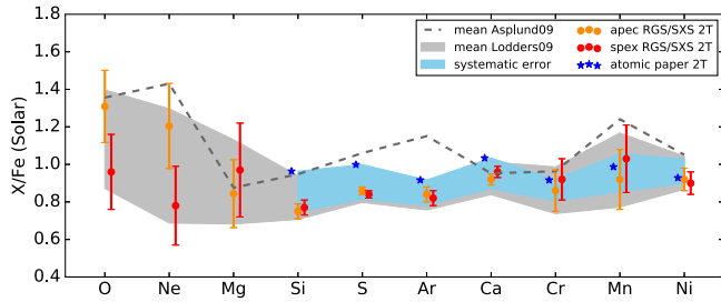
FIGURE 4 Abundance ratios measured for the Perseus cluster with XMM-Newton /RGS (O, Ne, Mg to Fe) and Hitomi /SXS (Si through Ni to Fe, Simionescu et al. 2019). The light blue strip is the systematic uncertainty on the Hitomi data. The grey strip includes both systematic and statistical uncertainties. The measured values are given with respect to the units of Lodders & Palme (2009) and Asplund et al. (2009).
