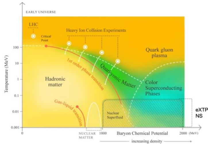
Figure 1. States of baryonic matter in the parameter space of temperature against baryon chemical potential. Note that 1-2 GeV corresponds to \sim 1 -6 times the density of normal atomic nuclei. Neutron stars access unique states of matter that cannot be created: nuclear superfluids, strange matter states with hyperons, deconfined quarks, and color superconducting phases.
