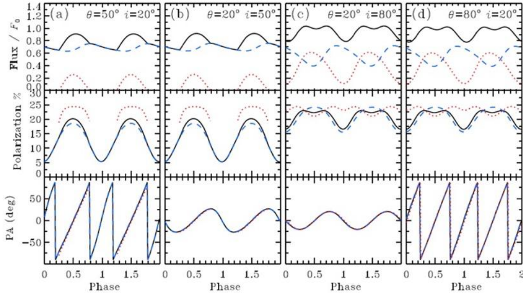
Figure 3. The pulse profiles as well as the phase dependence of the polarization degree (PD) and Polarization angle (PA) are shown. The black solid shows the contribution of two antipodal spots. Here i is the observer inclination and \theta is the hotspot colatitude. The pulse profiles and PD are degenerate with respect to i and \theta , while PA shows a dramatically different behavior so that both angles can be obtained. 17
