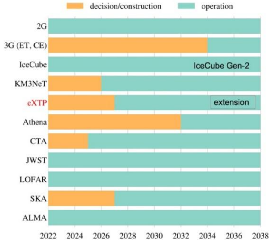
Figure 13. eXTP will operate in the epoch of truly multi-wavelength and multi-messenger astrophysics. 2G refers to second generation GW interferometers: aLIGO, Advanced Virgo, KAGRA and LIGO India. 3G refers to the third generation that will start in the mid thirties: Einstein Telescope and Cosmic Explorer. IceCube (and its extension Gen-2) and KM3NeT will significantly open neutrino astronomy. CTA is expected to be deployed soon and will boost our knowledge of the TeV Universe. LOFAR, SKA and ALMA are large enterprises in the radio and mm band. The large radio telescope FAST and ultra-high energy gamma-ray observatory LHAASO in China are operational, but not shown.
