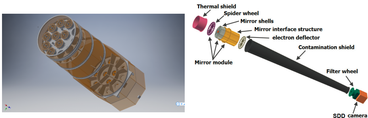
Figure 16. Left panel: Layout of the nine SFA telescopes (the four empty holes are reserved for PFA telescopes); Right panel: Schematic structure of one SFA telescope.
