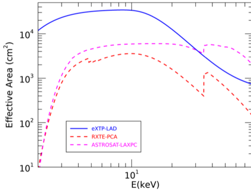
Figure 19. Comparison of the total effective area between LAD and other collimated X-ray telescopes.
