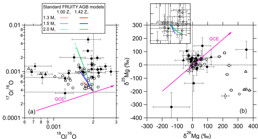
Fig. 6. A comparison of the same set of presolar spinel grains data as in Fig. 5 with the FRUITY model predictions of Cristallo et al. (2009, 2011) for low-mass RGB/AGB stars during the O-rich phase. Note that (i) the x and y axis ranges are narrower in both panels compared to Fig. 5 and (ii) different groups of grains from this study are all shown as filled symbols in black instead of in different colors as in Fig. 5. Panel b includes a subpanel that zooms into the FRUITY model region ( -20\% to 20\% in both x and y axes).
