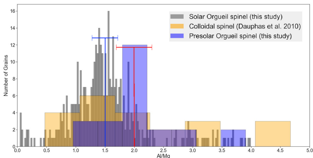
Fig. 4. A comparison of 24 O-anomalous spinel grains ( Table 1 ) with all other Al-rich grains in the same \text{Al}^+ ion images for their Al/Mg ratios. Also shown are the TEM-EDX Al/Mg ratios of Al-rich spinel grains from Orgueil and Murchison acid residues reported in Table 1 of Dauphas et al. (2010) . The Al/Mg data from this study were corrected for the Mg/Al RSF based on SRM 610 measurements. The red and blue lines represent the 15% 1\sigma errors in the determined Al/Mg ratio for Al/Mg ratios of 2 and 1.5, respectively.
