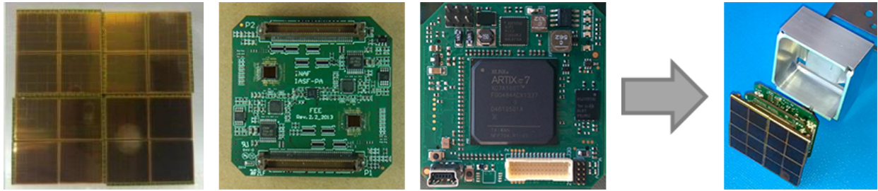
Figure 2. Components of the Photo Detection Module unit and its assembly
