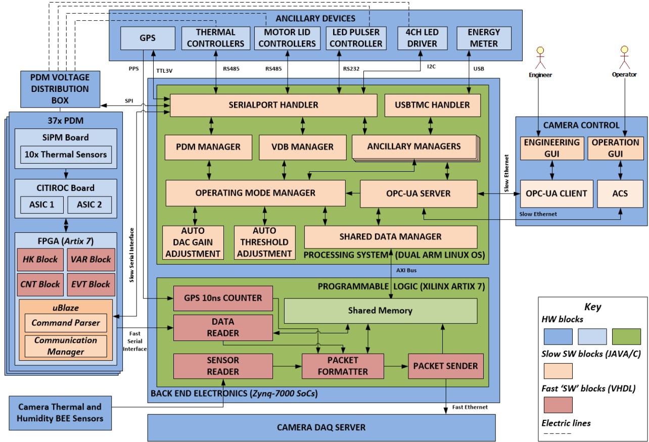
Figure 6. Astri SST-2M Camera Software Architecture
