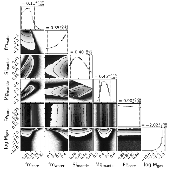
Figure 12. Posterior distributions of the most relevant internal structure parameters for TOI–757 b. The values above the histograms are the median and the 5th and 95th percentiles of the distributions, same as the dashed lines. The plotted internal structure parameters are the iron core and water mass fractions of the solid planet without gas, the molar fraction of Si and Mg within the mantle and of Fe in the core and the \log_{10} of the absolute gas mass in Earth masses.
