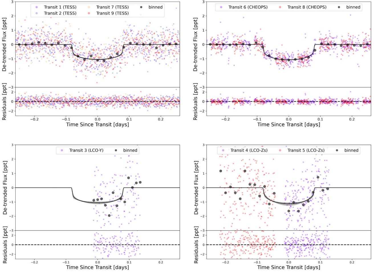
Figure 6. Detrended photometric light curves, folded over the best-fitting orbital period P , along with the best-fitting planet model and the posterior constraints corresponding to the 16 th and 84 th percentiles (see Section 5.1). The dotted data points are colour-coded to show the individual transits for each telescope. For clarity, we also overplot the binned detrended data in black dots. Top panel: TESS (left) and CHEOPS (right) folded light curves. Bottom panel: LCO–Y (left) and LCO–zs (right) folded light curves.
