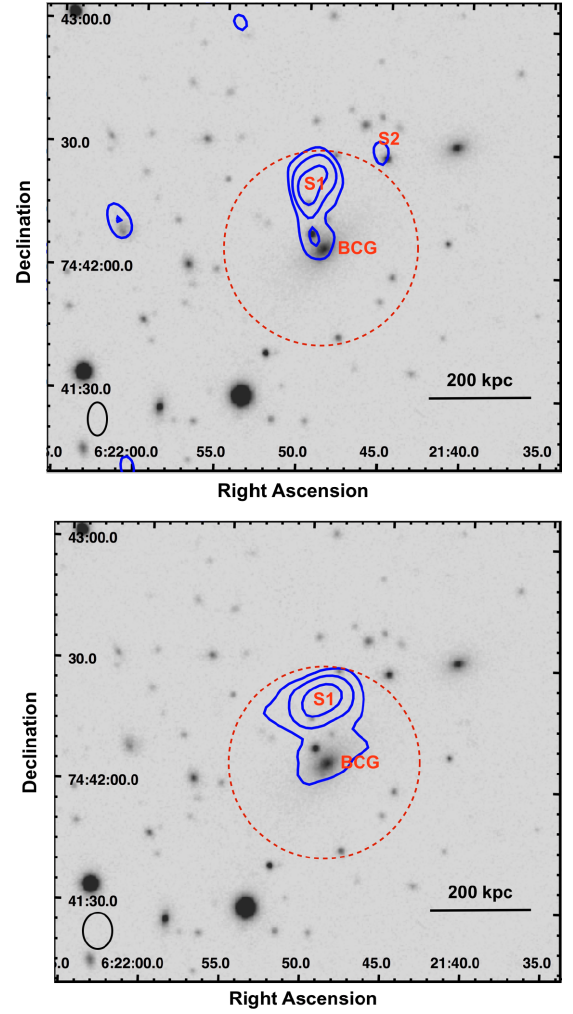
Figure 3. Optical Pan-STARRS image in grey-scale with the high resolution 610 MHz GMRT (top) and 144 MHz LOFAR (bottom) blue contours overlaid. The GMRT and LOFAR beam is 8.0 \text{ arcsec} \times 4.7 \text{ arcsec} and 8.0 \text{ arcsec} \times 6.5 \text{ arcsec} , respectively, and the GMRT and LOFAR levels are (2, 4, 8) \times 3\sigma , where \sigma = 27 \mu\text{Jy beam}^{-1} and \sigma = 140 \mu\text{Jy beam}^{-1} , respectively. The central radio components are indicated with labels: BCG is the BCG that corresponds also to the X-ray centre; S1 is a source that has no obvious optical counterpart, and is likely to be a background galaxy; S2 is a faint source that is not detected in the LOFAR image. The dashed-red region indicated the core region of the cluster, which has a size of \sim 200 \text{ kpc} .
