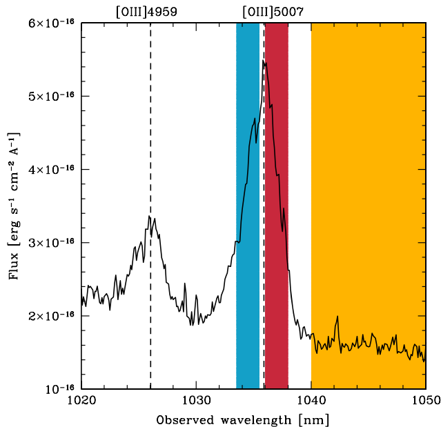
Figure 2. Left: Keck/OSIRIS spectrum of the region of the [O III]4959,5007 doublet extracted from a region of r = 6 spaxels ( r = 0''.6 ) centered on the centroid of the continuum source. The colored areas refer to the collapsed images shown in the right panel. Dashed lines indicate the redshifted wavelengths of the lines at the systemic redshift z_s = 1.0685 . Right: Keck/OSIRIS collapsed images of three different spectral regions. We show that the continuum emission between 1040 and 1150 nm (top, yellow shaded area in the left figure), continuum-subtracted blue side of the [O III]5007 line between 1033.5 and 1035.5 nm (center), and continuum-subtracted red side of the same line between 1036 and 1038 nm (bottom). The green circles in the center and bottom panels indicate the centroid of the continuum source.
