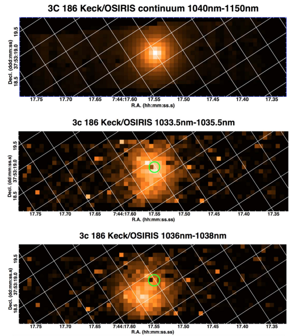
Figure 2. Left: Keck/OSIRIS spectrum of the region of the [O III]4959,5007 doublet extracted from a region of r = 6 spaxels ( r = 0''.6 ) centered on the centroid of the continuum source. The colored areas refer to the collapsed images shown in the right panel. Dashed lines indicate the redshifted wavelengths of the lines at the systemic redshift z_s = 1.0685 . Right: Keck/OSIRIS collapsed images of three different spectral regions. We show that the continuum emission between 1040 and 1150 nm (top, yellow shaded area in the left figure), continuum-subtracted blue side of the [O III]5007 line between 1033.5 and 1035.5 nm (center), and continuum-subtracted red side of the same line between 1036 and 1038 nm (bottom). The green circles in the center and bottom panels indicate the centroid of the continuum source.
