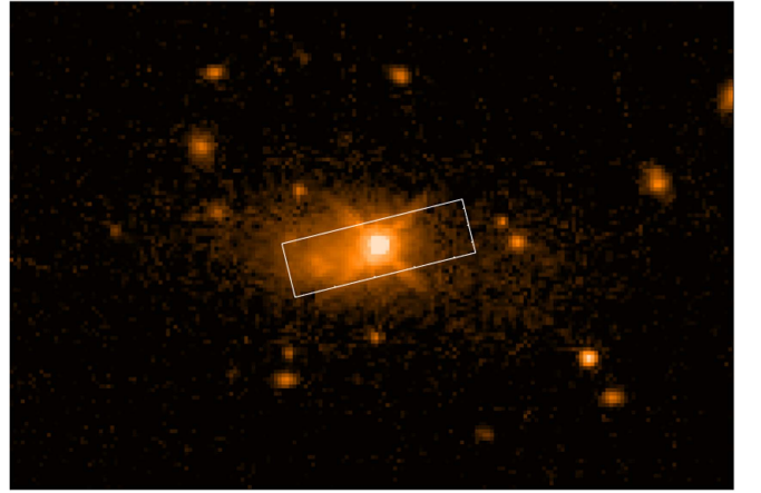
Figure 1. OSIRIS field of view ( 1''.6 \times 6''.4 , corresponding to \sim 13 \text{ kpc} \times \sim 52 \text{ kpc} , at the distance of the target) overlaid onto the HST /WFC3-IR F140W image of 3C 186 (adapted from Chiaberge et al. 2017).
