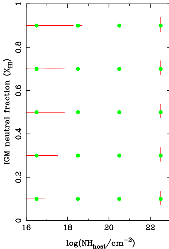
Fig. 9 Results of simulations showing how well the IGM neutral fraction \chi_{\text{HI}} and host H I column density can be retrieved from typical ELT-class afterglow spectra (cf. Fig. 5). The input values are shown as green points, and the resultant fits by the red contours. In nearly all cases the IGM neutral fraction is well recovered (within the symbol size), as are host columns for all but the lowest cases, although even here results should be sufficient to indicate a partially transparent sight line. The variance between sight-lines at the same redshift of IGM neutral fraction is expected to be up to \delta\chi_{\text{HI}} \sim 0.3 at mid reionization [107, 108], depending on the reionization model, which can be determined with the THESEUS sample
