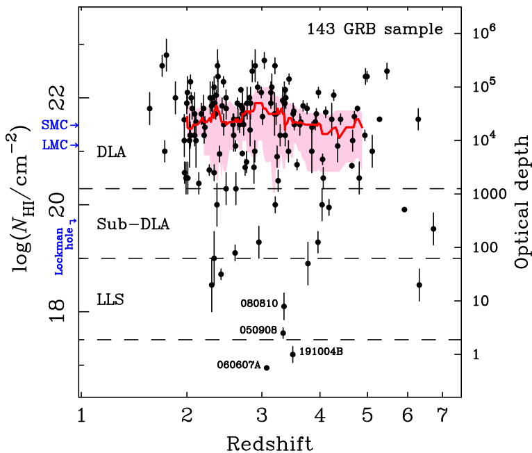
Fig. 7 The host neutral hydrogen column densities measured from the \text{Ly}\alpha absorption line in the afterglows of 143 GRBs spanning a wide range of redshift. Typically, the columns imply a high optical depth to ionizing Ly-continuum radiation, and thus a low overall escape fraction ( f_{\text{esc}} < 2\% ). Strikingly, there is little evolution in the running median value (red line) or inter-quartile range (pink region) over the redshift for which the distribution is well sampled, but there is a hint of a possible downturn at the highest redshifts. THESEUS will enable us to extend this plot with good statistics at z > 5 providing a direct estimate of the escape fraction on the lines of sight to massive stars in this era
