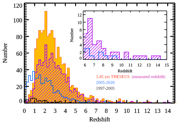
Fig. 1 A realisation of the expected redshift distribution of long-duration GRBs detected by THESEUS in 3.45 yr of scientific operations (orange and purple histograms) based on GRB population modeling [40], compared with the redshift distribution obtained to date (blue and black histograms)
