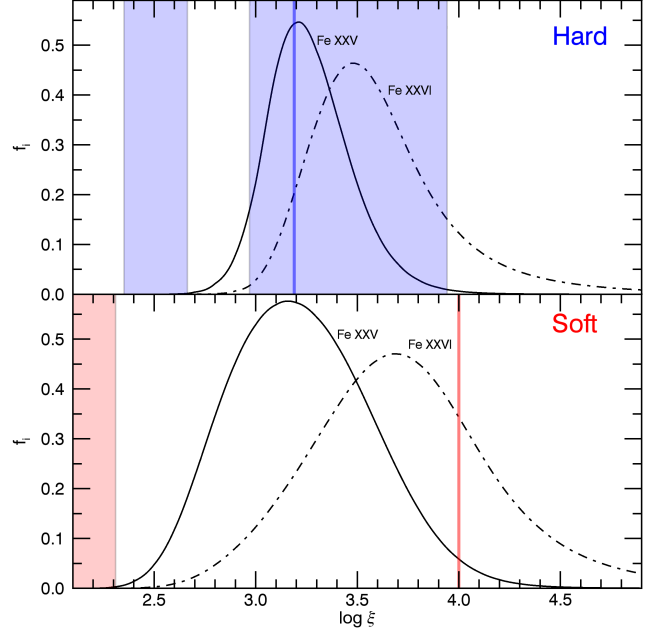
Figure 4. Ionic fractions for Fe XXV and Fe XXVI, when the illuminating SED is that of the hard ( top ) and soft ( bottom ) state. The red vertical solid line marks the best-fitting value of the ionization parameter for the observed plasma in the soft state as found by Pontì et al. (2015), while the blue vertical solid line the value of the ionization parameter in the hard state, assuming that its physical properties did not change ( nr^2 = \text{const} ). The shaded blue and red bands are the ionization parameter's ranges where the plasma is in the unstable parts of the stability curves shown in Fig. 3.
