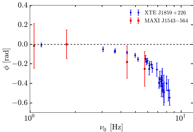
Figure 9. Type-C fundamental phase lags as a function of the QPO frequency for XTE J1859+226 and MAXI J1543-564, both sources of undetermined inclination. Both sources show significant hard lags, consistent with the high-inclination sample.
