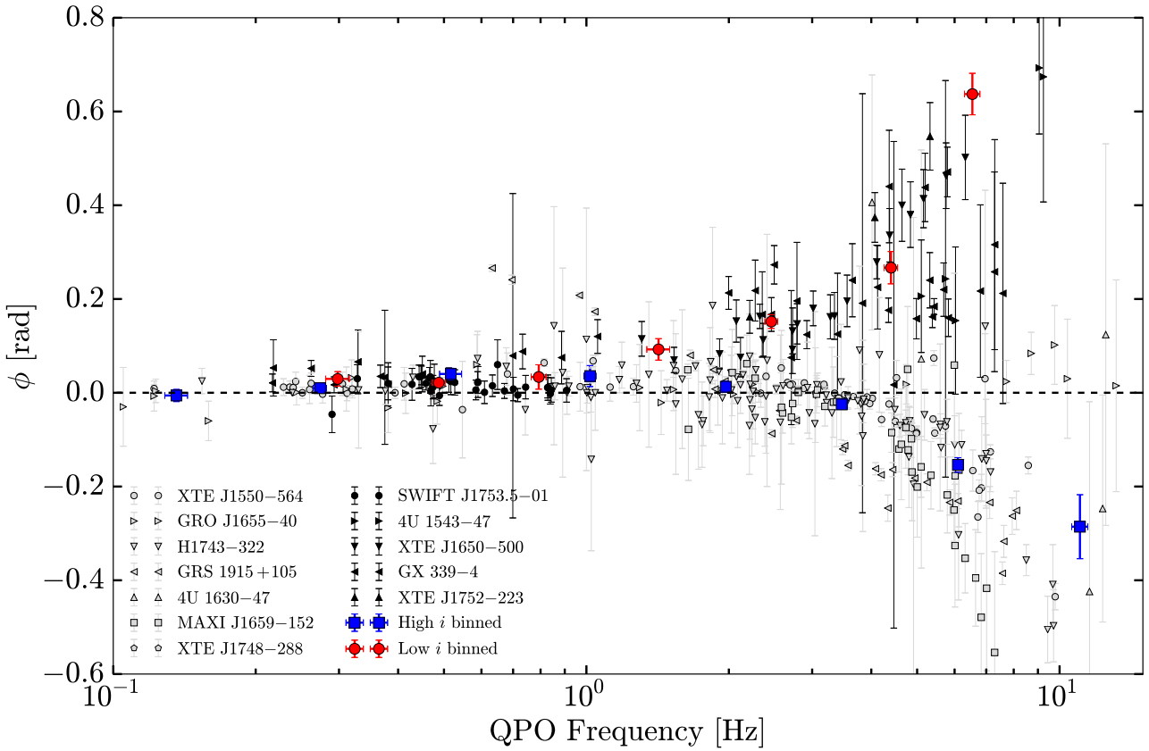
Figure 3. Type-C QPO phase lags as a function of the QPO frequency. Black and grey points indicate low- and high-inclination sources, respectively. Different sources within the low- or high-inclination sample are shown with different markers. The red and blue points show the average phase lag and the QPO frequency in logarithmic frequency bins. The plots for individual sources, including the two sources of unknown inclination, can be found in Appendix A.
