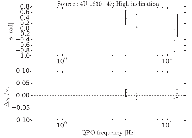
Figure A9. Type-C QPO phase lag and \Delta\nu_0/\nu_0 as a function of the QPO frequency for 4U 1630–47.
