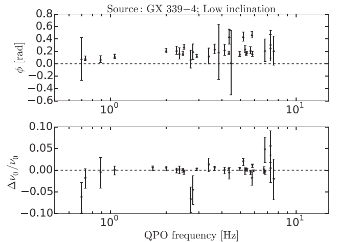
Figure A4. Type-C QPO phase lag and \Delta\nu_0/\nu_0 as a function of QPO frequency for GX 339–4.
