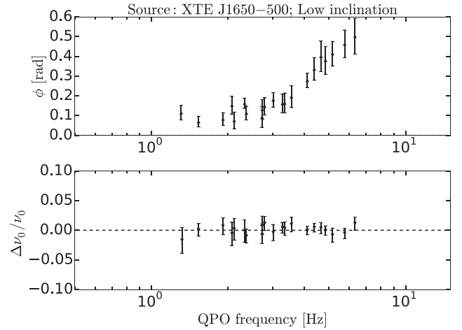
Figure A3. Type-C QPO phase lag and \Delta\nu_0/\nu_0 as a function of the QPO frequency for XTE J1650–500.
