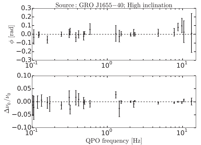
Figure A10. Type-C QPO phase lag and \Delta\nu_0/\nu_0 as a function of the QPO frequency for GRO J1655–40.
