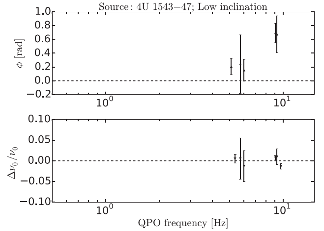
Figure A2. Type-C QPO phase lag and \Delta\nu_0/\nu_0 as a function of the QPO frequency for 4U 1543–47.
