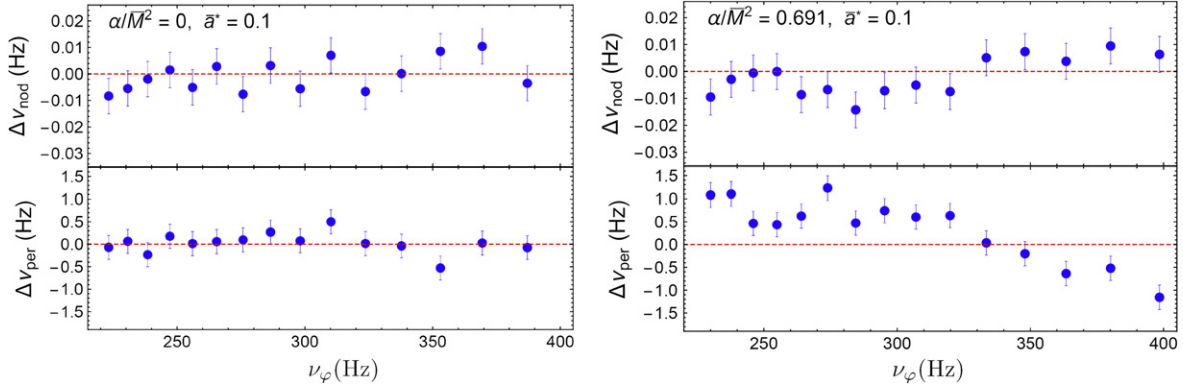
Figure 5. \Delta\nu_{\text{nod}} = (\nu_{\text{nod}} - \hat{\nu}_{\text{nod}}) and \Delta\nu_{\text{per}} = (\nu_{\text{per}} - \hat{\nu}_{\text{per}}) are shown as functions of the azimuthal frequency \nu_\phi for BH configurations with \bar{M} = 5.3M_\odot , \bar{a}^* = 0.1 , and coupling parameter \alpha/\bar{M}^2 = (0, 0.691) . \hat{\nu}_{\text{per,nod}} correspond to the periastron and nodal frequencies computed for the best-fit parameters (\hat{M}, \hat{a}^*) , which have been obtained by minimizing the chi-square variable (28). The error bar is 1\sigma .
