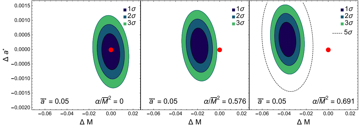
Figure 3. Confidence levels with which GR can be tested against the EDGB theory (see the text) are plotted in the (\Delta M, \Delta a^*) plane. The red dot is the origin of the plane. The parameters corresponding to the two injected sets of frequencies (\nu_\varphi, \nu_{\text{per}}, \nu_{\text{nod}})_j are \bar{r}_j/\eta_{\text{SCO}} = 1.1, 1.4 , \bar{M} = 5.3 M_\odot , and \bar{a}^* = 0.05 . Remember that these frequencies are computed using the EDGB theory. In the left panel, we assume that the coupling constant of the EDGB theory, \alpha/\bar{M}^2 , is zero, so that the EDGB theory coincides with GR. The red dot falls in the center of the 1\sigma ellipse, showing that the two sets of frequencies are fully compatible with GR and that our statistical analysis is correct. In the right panel, we set \alpha/\bar{M}^2 = 0.691 , i.e., the maximum value allowed by the EDGB theory. The red dot is well outside the 5\sigma confidence level (dashed line), showing that in this case we would be able to exclude that the two sets of frequencies are generated according to GR. In the middle panel, \alpha/\bar{M}^2 = 0.576 and the red dot touches the 3\sigma confidence level, i.e., the frequencies would be incompatible with GR to this confidence level.
