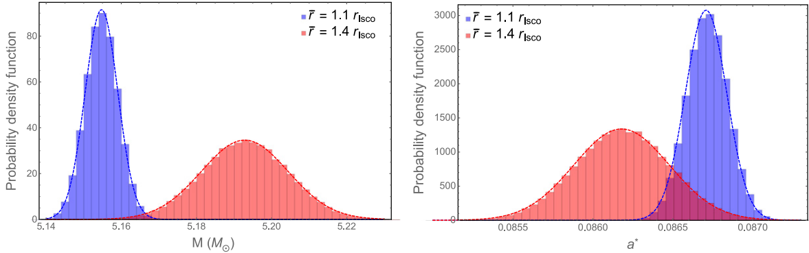
Figure 2. Distribution of the BH mass M (left panel) and spin a^* (right panel) as obtained from the measurement of the epicyclic frequencies ( \nu_{\varphi} , \nu_{\text{per}} , \nu_{\text{nod}} ) at two different radii r . The generated frequencies follow Gaussian distributions with relative widths 15 times lower than those measured with the RXTE /PCA from GRO J1655-40, as expected for the LOFT -LAD instrument. A BH mass \bar{M} = 5.3 M_{\odot} and spin parameter \bar{a}^* = 0.1 are adopted here in EDGB gravity with the maximal coupling constant ( \alpha/\bar{M}^2 = 0.691 ).
