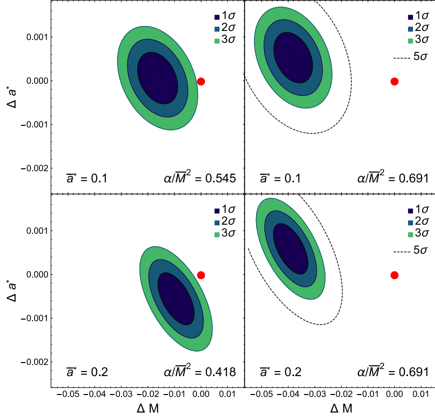
Figure 4. Same as Figure 3, with \bar{a}^* = 0.1, 0.2 (upper and lower panels, respectively). \alpha/\bar{M}^2 has the maximum value in the right panels, and the threshold value for which GR would be excluded at 3\sigma confidence level in the left panels.
