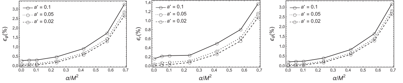
Figure 1. Relative difference between the azimuthal/epicyclic frequencies ( \nu_{\varphi} , \nu_r , \nu_{\theta} ) computed in GR and in the EDGB theory plotted as a function of the coupling constant \alpha/M^2 for different values of the BH spin parameter a^* = (0.02, 0.05, 0.1) . All quantities are computed at r = 1.1 \eta_{\text{ISCO}} .
