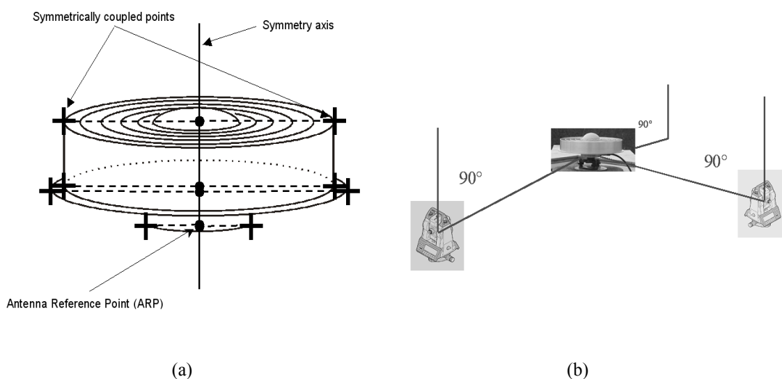
Fig. 3: a) Scheme of measured points with respect to the GPS antenna vertical axis. b) Triangulation scheme of the GPS ARP performed from tripods of the ground control network.
