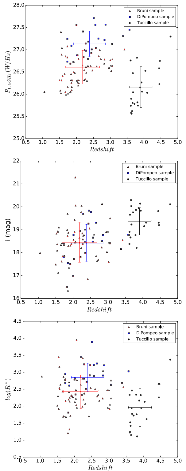
Figure 1. We show, as a function of the redshift, the distributions in radio luminosity [at \log_{10} P_{1.4\text{GHz}} (\text{W Hz}^{-1}) ], i -magnitude and radio-loudness R for the 25 RL BAL QSOs (red triangles) used in Bruni et al. (2012), for the 74 RL BAL QSOs (blue squares) used in DiPompeo et al. (2011) and for the 22 RL BAL QSOs (black dots) used in this work. The large crosses with the 1\sigma error bar represent the location of the mean for each of the plotted samples. The sample studied in this work was selected in order to extend the previous cited studies at higher redshift and at lower optical and radio fluxes, probing new parameter space. See Section 2.1.
