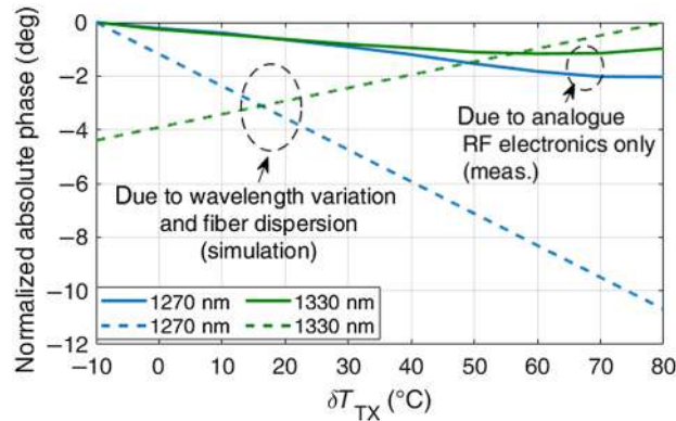
Fig. 15 Normalized absolute phase variation with respect to FEM operative temperature \delta T_{TX} normalized (to their max values) at 160 MHz for both RF1 and RF2 considering only the analogue RF electronics (solid lines) and the one expected due to temperature-induced wavelength-shift and fiber dispersion (dashed lines).
