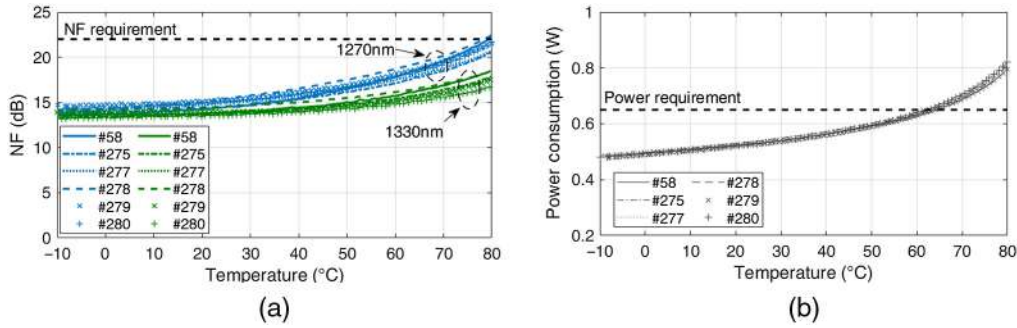
Fig. 11 Examples of receiver verification measurements versus FEM temperature: (a) noise figure (NF) at 160 MHz (the measurements include 6 km of SMF fiber between FEM and PREADU at ambient temperature) and (b) FEM power consumption. The causes which lead to the higher NF in the 1270 nm link are discussed in Sec. 3.2.1.
