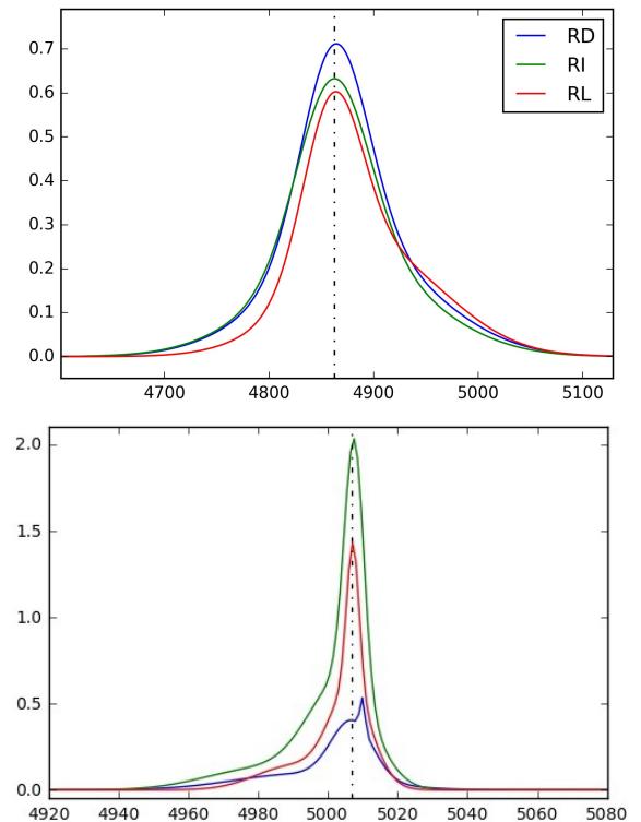
Fig. 8. CD B1 \text{H}\beta (top) and CD A2 [\text{OIII}] profiles (bottom) for different radio power classes. Blue refers to the RD class, green to the RI one and red to the RL one.
