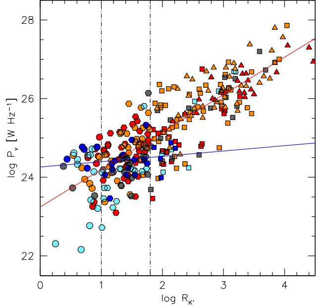
Fig. 11. Behavior of radio power P_\nu in units of W as a function of the Kellermann's parameter R_K . Symbol coding corresponds to different radio morphologies and to different STs. Triangles: RL FR II; squares: RL CD, exagons: CD RI, circles: CD RQ. Red: union of \text{B1}^{++} and \text{B1}^+ , orange: B1, gray: A1, pale blue: A2, xA: blue. The lines trace unweighted least square fits for Pop. B sources (red) and for xA sources considered over the three radio loudness classes.
