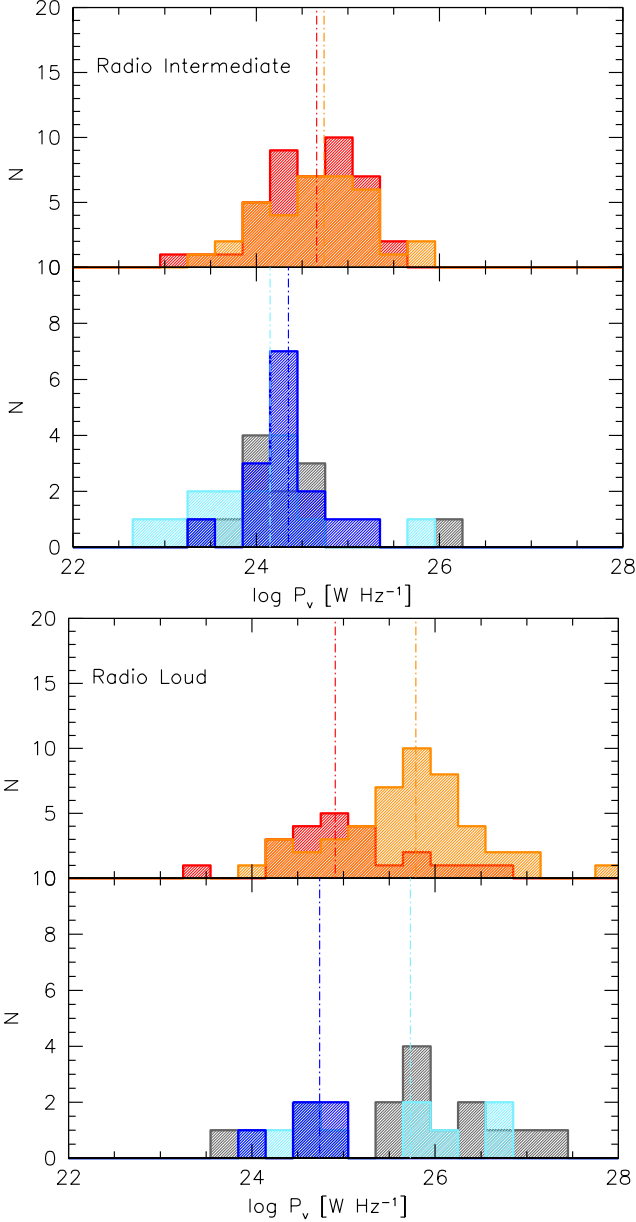
Fig. 10. Distribution of radio power P_\nu in units of W for RI (top) and RL (bottom), for different spectral types along the main sequence. The top panels show the distributions for the union of \text{B1}^{++} and \text{B1}^+ (red), B1 (orange) spectral types, the bottom ones for A1 (gray), pale blue (A2), and xA (blue). The vertical dot-dashed lines mark the medians of the Pop. B (red and orange), A2 (pale blue) and xA (blue) distributions.
