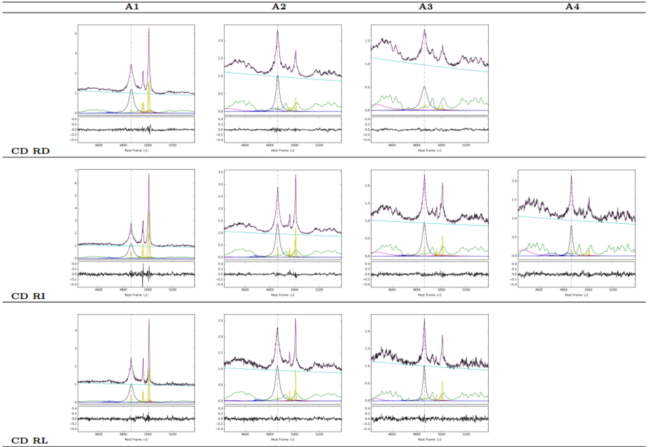
Fig. 4. Composite of spectral types along the MS, ordered from A1 to A4. Color scheme same as in Fig. 3.
