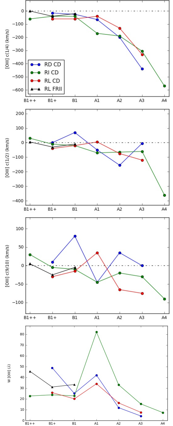
Fig. 6. CD [OIII] centroid shifts (km/s) for different E1 classes and for different line height. From top to bottom: x = 1/4 , x = 1/2 , x = 9/10 . Bottom: equivalent width ( \text{\AA} ) distribution. Blue refers to the RD class, green to the RI one and red to the RL one.
