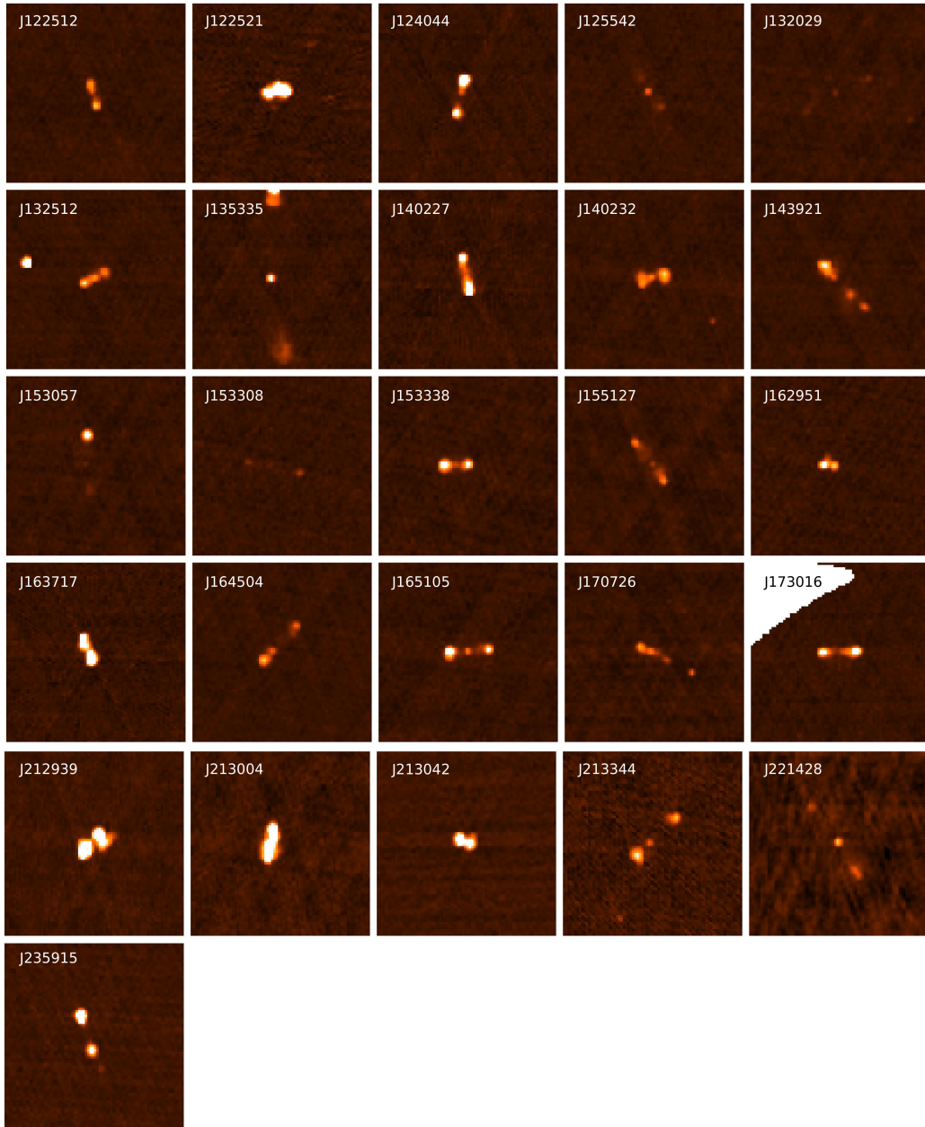
Fig. B.1. Radio maps at 1.4 GHz for the FRII sample from the FIRST catalog with size of field 4.5' \times 4.5' and a Maximum Intensity for Scaling equals to 10 mJy. The images follow the SDSS ID order of table A.2 from left to right and from top to bottom.
