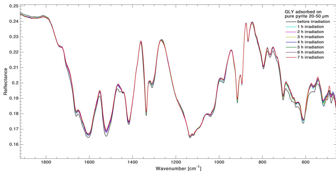
FIGURE 5 | Superimposition of infrared spectra of GLY adsorbed on pyrite in the range 2,000–500 \text{cm}^{-1} during 7 h of UV irradiation. Spectra were collected in situ at 1-h intervals to monitor the kinetics of degradation in real time.
