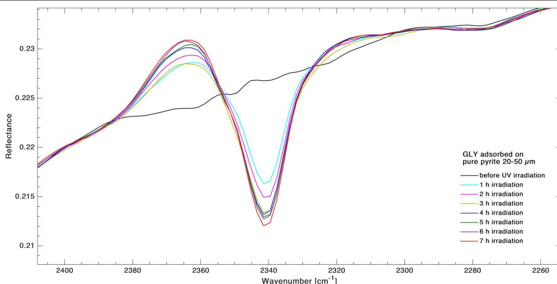
FIGURE 6 | Superimposition of infrared spectra of GLY adsorbed on pyrite for forming band at 2,340\text{ cm}^{-1} during 7 h of UV irradiation. Spectra were collected in situ at 1-h intervals to monitor the kinetics of degradation in real time. The growing band area of \text{CO}_2 band is clearly visible.
