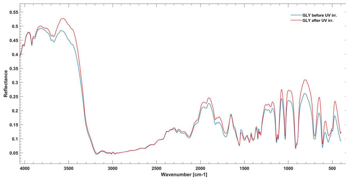
FIGURE 4 | Infrared spectrum of pure GLY in the range 4,000–400 \text{cm}^{-1} before (blue line) and after (red line) 61.5 h of UV irradiation.
