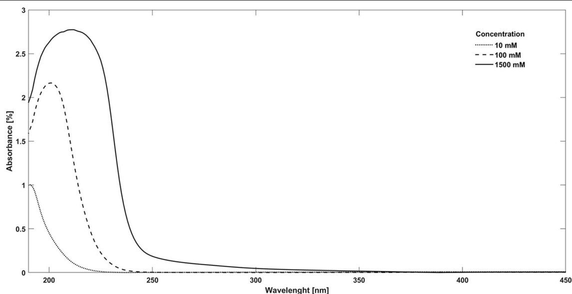
FIGURE 1 | Water-glycine adsorption UV spectra at various concentrations: dotted line, 10 mM; dashed line, 100 mM; and continuous line, 1,500 mM.
