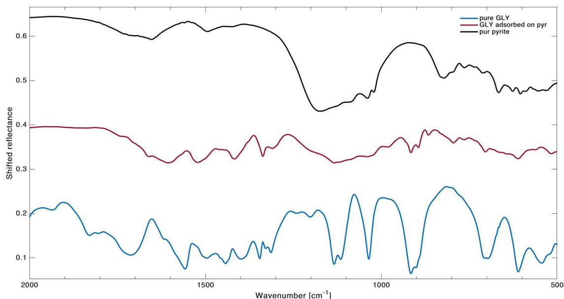
FIGURE 3 | Detail of spectra in wavenumber range 2,000–500 \text{cm}^{-1} with comparison between pure GLY (blue line), pure pyrite (black line, shifted 0.3 to the top), and GLY adsorbed on pyrite (red line, shifted 0.15 to the top).
