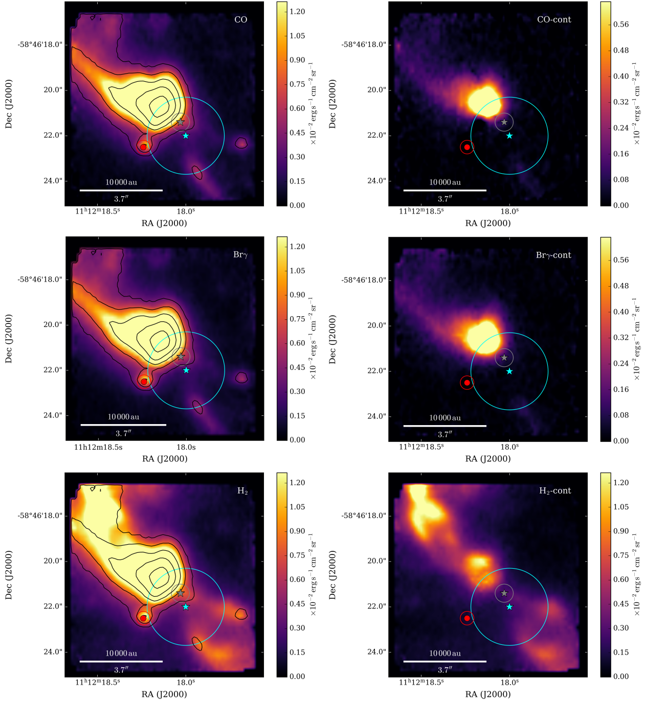
Fig. 3. Emission maps from VLT/SINFONI for CO (top), Br \gamma (middle), and H _2 (bottom), integrated over the peak of each line ( \Delta\lambda \sim 0.00024\mu\text{m} ). Left panels: the black contour lines represent the continuum emission at 2.08559\mu\text{m} , the levels are (5, 10, 20, 40, 80, 160) \times \sigma where \sigma \sim 0.1 \text{ erg s}^{-1} \text{ cm}^{-2} \mu\text{m}^{-1} \text{ sr}^{-1} . Right panels: represent the continuum-subtracted emission maps, where the continuum subtraction was performed by considering the continuum left (blue-shifted) and right (red-shifted) of each emission line, with the exception of the CO, where only the left (blue-shifted) part was considered. The red circle represents the star in the Gaia DR2 catalogue (Source ID: 5339406246100053888, RA(J2000) = 11^{\text{h}}12^{\text{m}}18.24^{\text{s}} , Dec(J2000) = -58^{\circ}46'22.5'' ) used for accurate astrometry of our cubes (the circle around it represents the uncertainty \sim 0.3'' ). The cyan star represents the suggested position of the star given by Tamura et al. (1997); the circle around it represents the uncertainty \sim 1.7'' . The grey star represents the position of the central source as given by our kinematic study (see Sect. 3.4). In all panels north is up and east is left.
