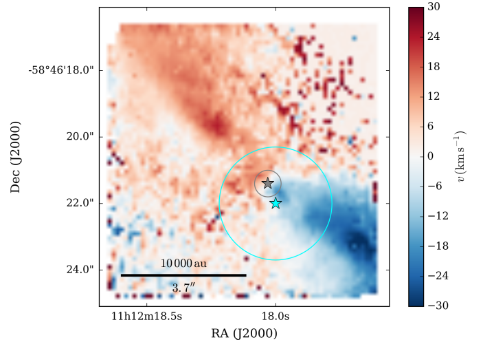
Fig. 5. Velocity map (LSR) of molecular hydrogen obtained from the 1–0 S(1) line at 2.12\mu\text{m} . The cyan star denotes the position of the star given by Tamura et al. (1997); the circle around it represents the uncertainty \sim 1.7'' . The grey star indicates our suggested position of the central engine; the circle around it represents the uncertainty \sim 0.4'' .
