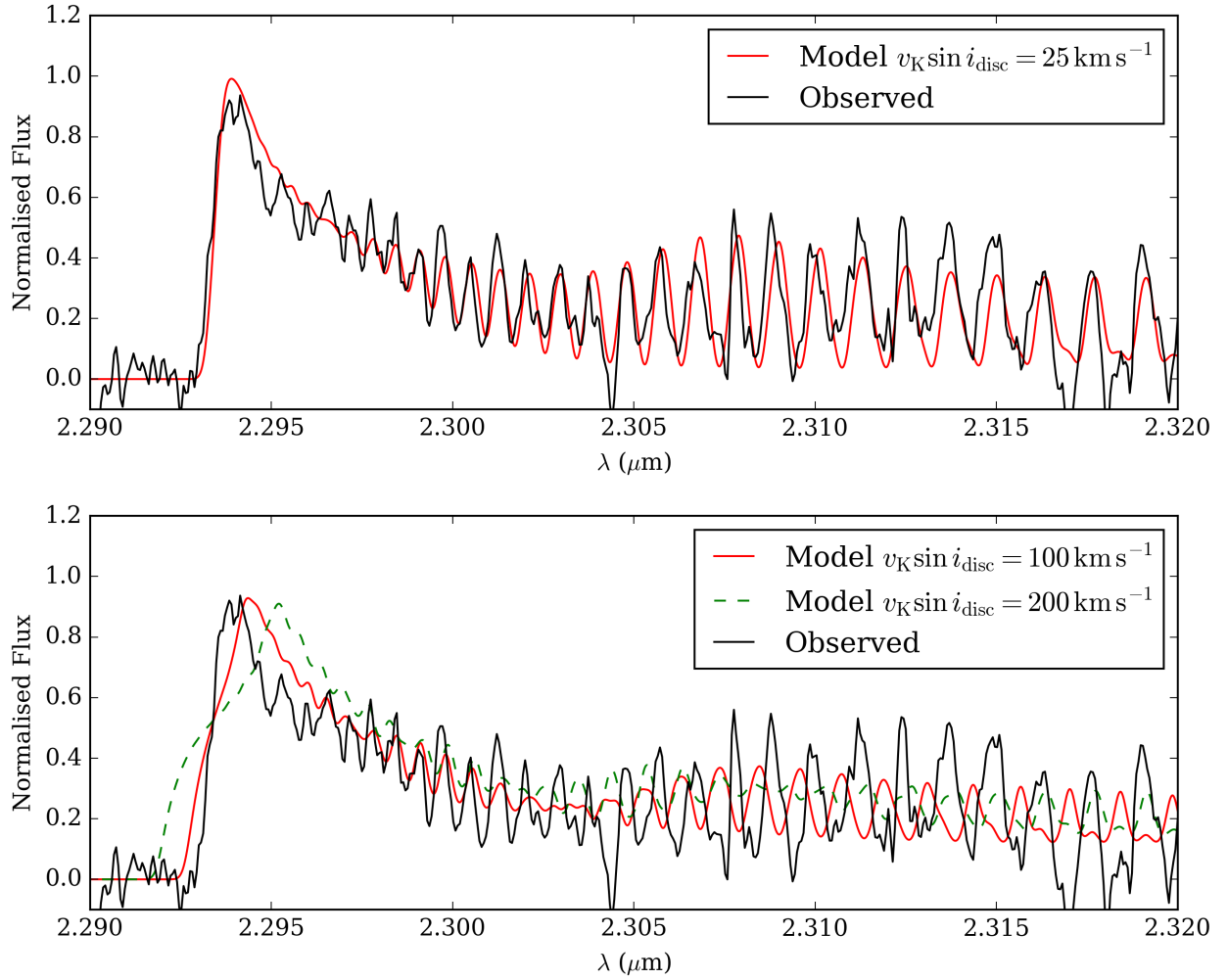
Fig. A.1. Top panel: VLT/X-shooter spectrum of the first CO bandhead emission (black) and the LTE model spectrum (red) obtained for T = 3000 \text{ K} , N(\text{CO}) = 1 \times 10^{22} \text{ cm}^{-2} , v_K \sin i_{\text{disc}} = 25 \text{ km s}^{-1} , and \Delta v = 10 \text{ km s}^{-1} . Bottom panel: same as top panel but with v_K \sin i_{\text{disc}} = 100 \text{ km s}^{-1} (red solid line) and 200 \text{ km s}^{-1} (green dashed line).
