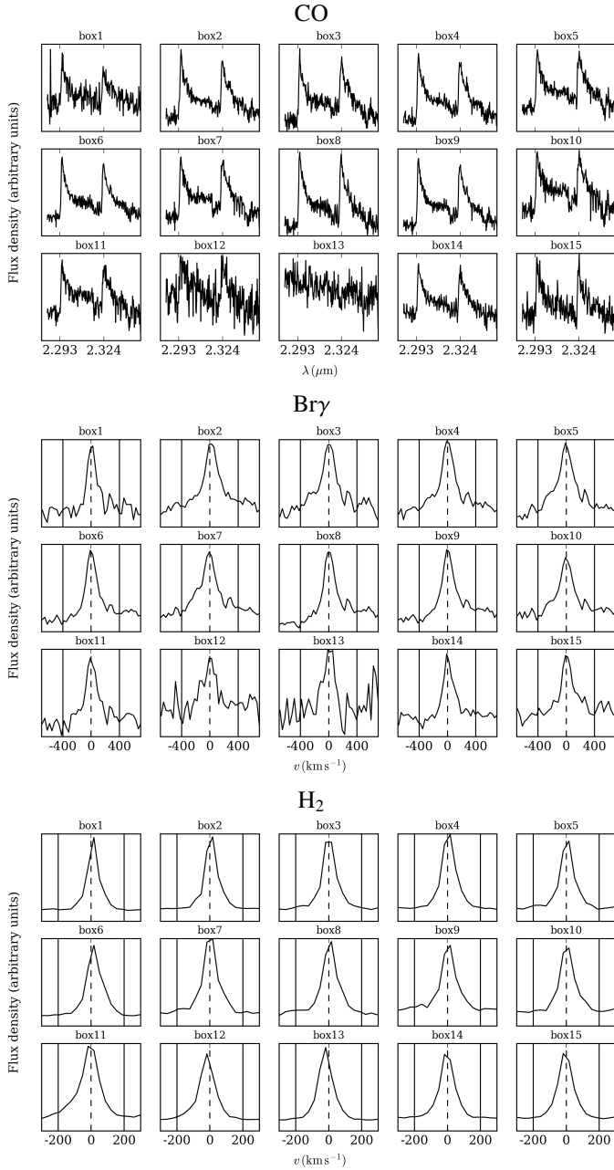
Fig. 4. Top panel: spectra from VLT/SINFONI showing the profile variation of the two firsts CO bandhead lines along the cube. Middle panel: same as top panel for the Br \gamma line at 2.16\mu\text{m} . Bottom panel: same as top panel for the H _2 line 1–0 S(1) at 2.12\mu\text{m} . The box numbering corresponds to that given in Fig. 1. Velocities are given with respect to the LSR.
