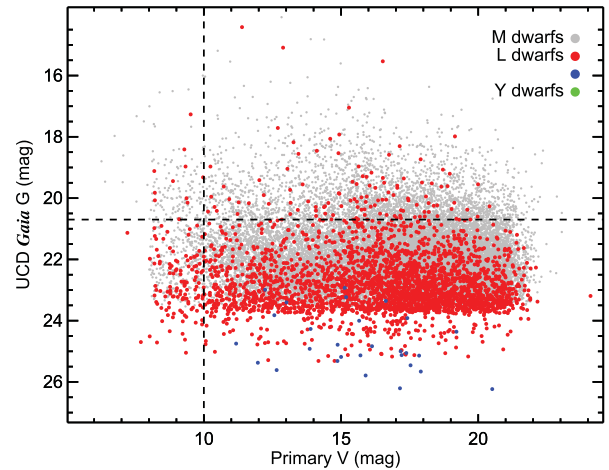
Figure 6. The Gaia G -band magnitudes of CGBs versus V -band primary magnitudes, with UCD spectral types coloured as in Fig. 1. Dashed lines indicate the Hipparcos limit ( V \sim 10 \text{ mag} ) for the primaries, and the Gaia G detection limit for the CGBs.
