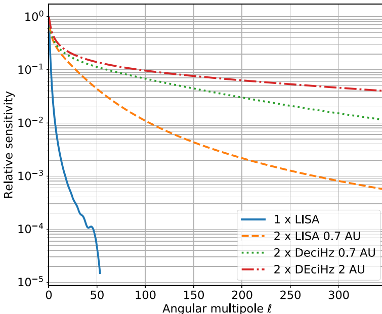
Fig. 2 Idealised angular resolution for different detector configurations (see text). The relative sensitivity to different angular multipoles is obtained by integrating the spherical response to a cross-correlation baseline weighted by a simple model of the noise spectrum based on the individual detector arm lengths. Convolution with the detector response functions and the sky-phase coverage would give additional structure on top of the idealised case
