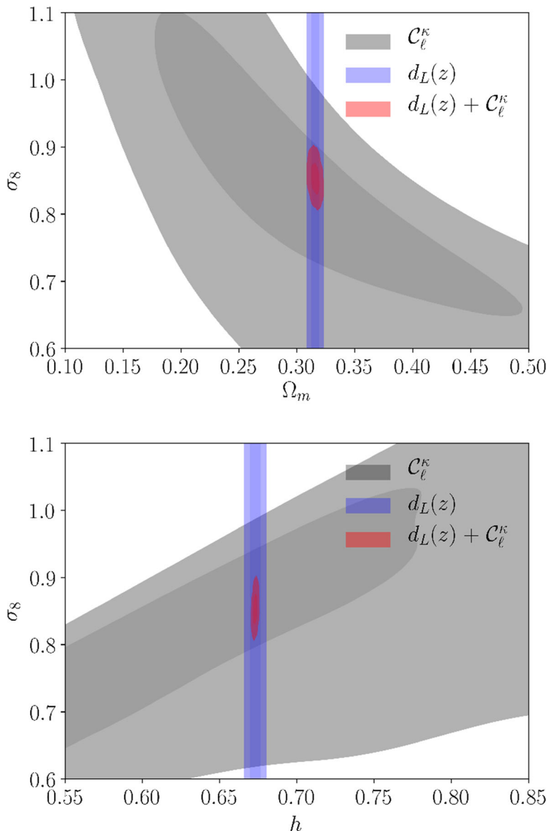
Fig. 1 Adapted from Fig. 1 of Ref. [38], cosmological forecast for the flat \Lambda CDM model assuming a very conservative source number density of 1 \text{ deg}^{-2} . The figure shows the constraints from luminosity distance only, d_L , the weak lensing convergence power spectrum, \mathcal{C}_\ell^\kappa , and jointly. Decihertz arcmin resolution would guarantee up to a factor of 50 improvement in number density (likewise for shot noise), hence allowing access to non-linear scales. The constraining power would be improved almost surely by an order of magnitude
