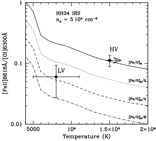
Fig. 10. [\text{Fe II}] 8616 \text{ \AA} / [\text{O I}] 6300 \text{ \AA} ratio plotted against the gas temperature for a density of 5 \times 10^4 \text{ cm}^{-3} . The solid curve shows predictions assuming an [\text{Fe/O}] solar gas phase abundance of 0.062 (Asplund et al. 2006). Other curves are plotted for decreasing values of the [\text{Fe/O}] abundance. Data points correspond to the values measured in the HVC and LVC toward HH34 IRS, and indicate an [\text{Fe/O}] abundance ratio close to solar for the HVC and a factor between 2 and 8 below solar for the LVC.
