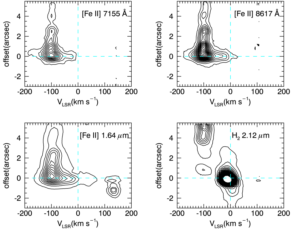
Fig. 5. As in Fig. 3 but for [Fe II] and the H 2 2.12 \mu\text{m} lines. Contours start at 3\sigma and are drawn at steps of 3\sigma , with the exception of 1.64 \mu\text{m} where the first five contours are at 2, 4, 6, 8, and 10\sigma to emphasize the red-shifted emission, and then continue at steps of 6\sigma .
