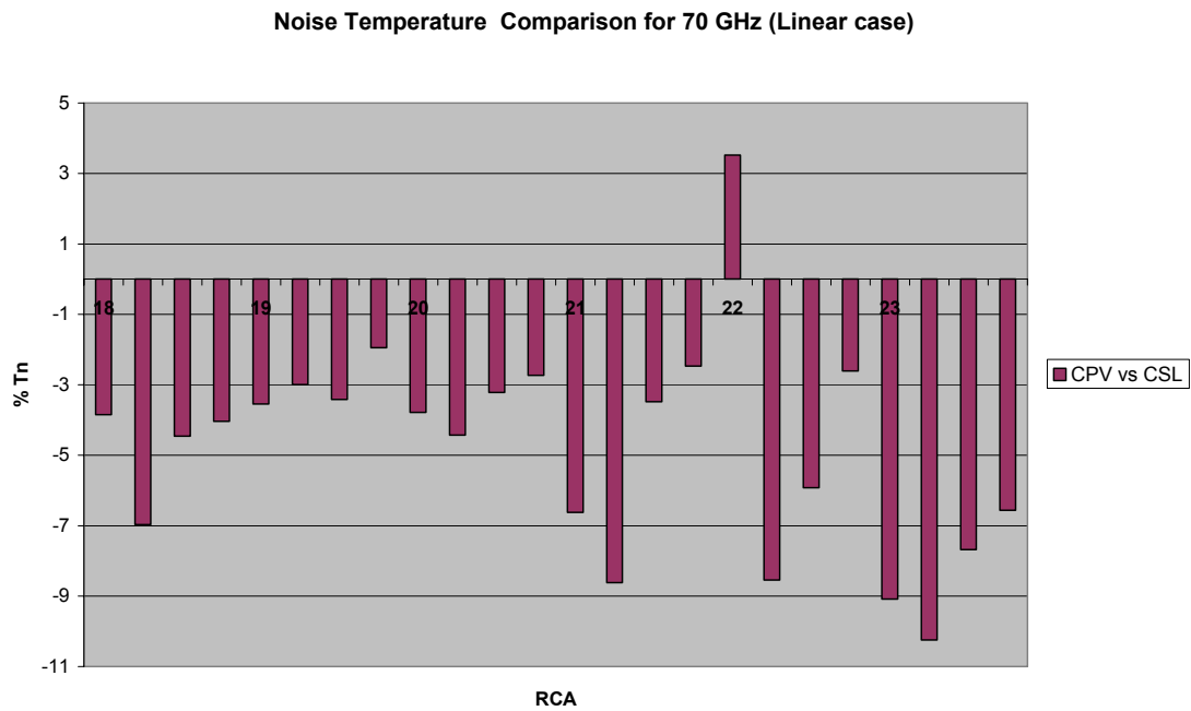
Plot 2 Noise Temperature comparison at 70 GHz between CPV and CSL optimal bias using a linear model of the radiometer. The percent variation is displayed on Y axis.
